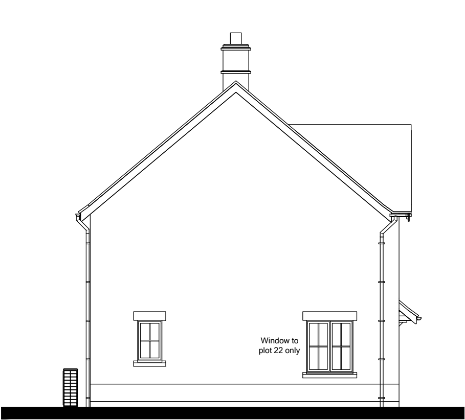
Side Elevation
