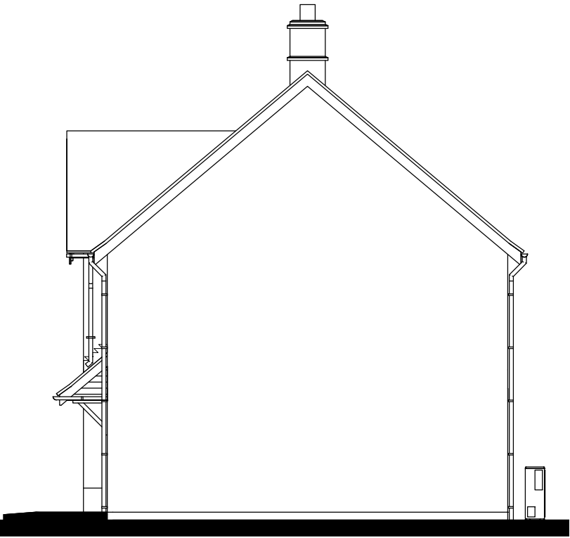
Side Elevation
