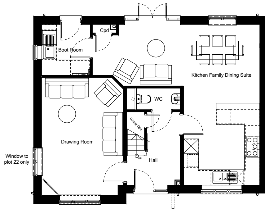
House Type D - Ground Floor Plan
