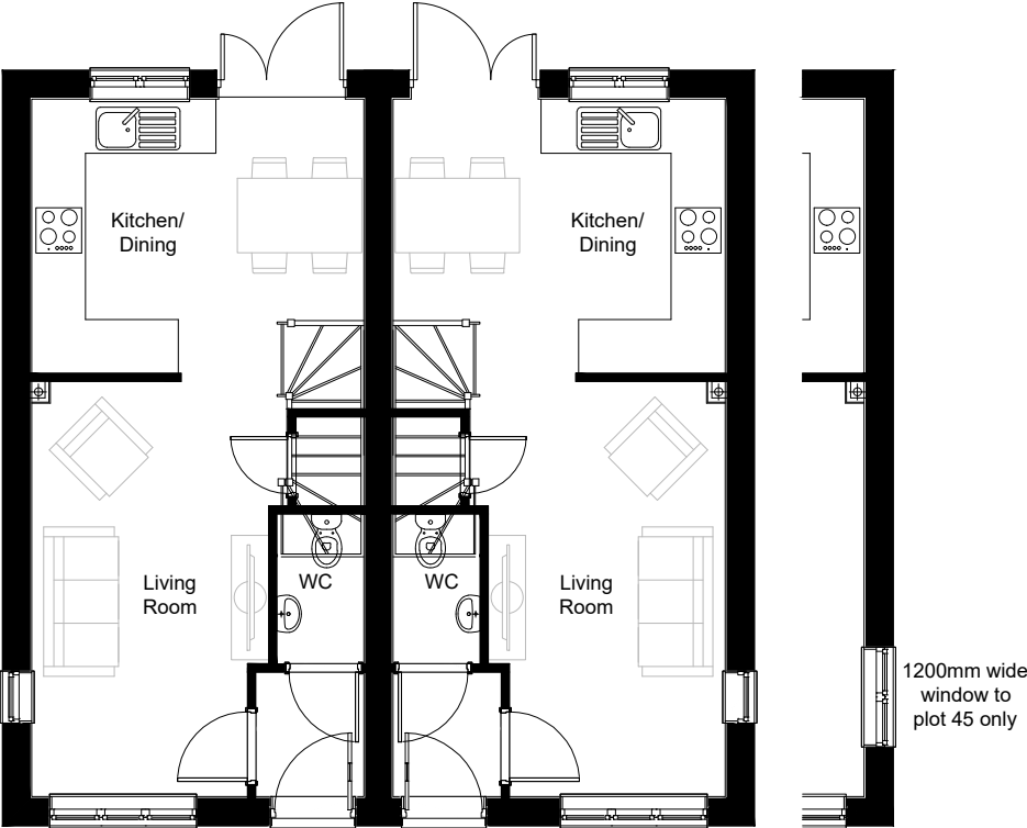
House Type A2 - Ground Floor Plan
