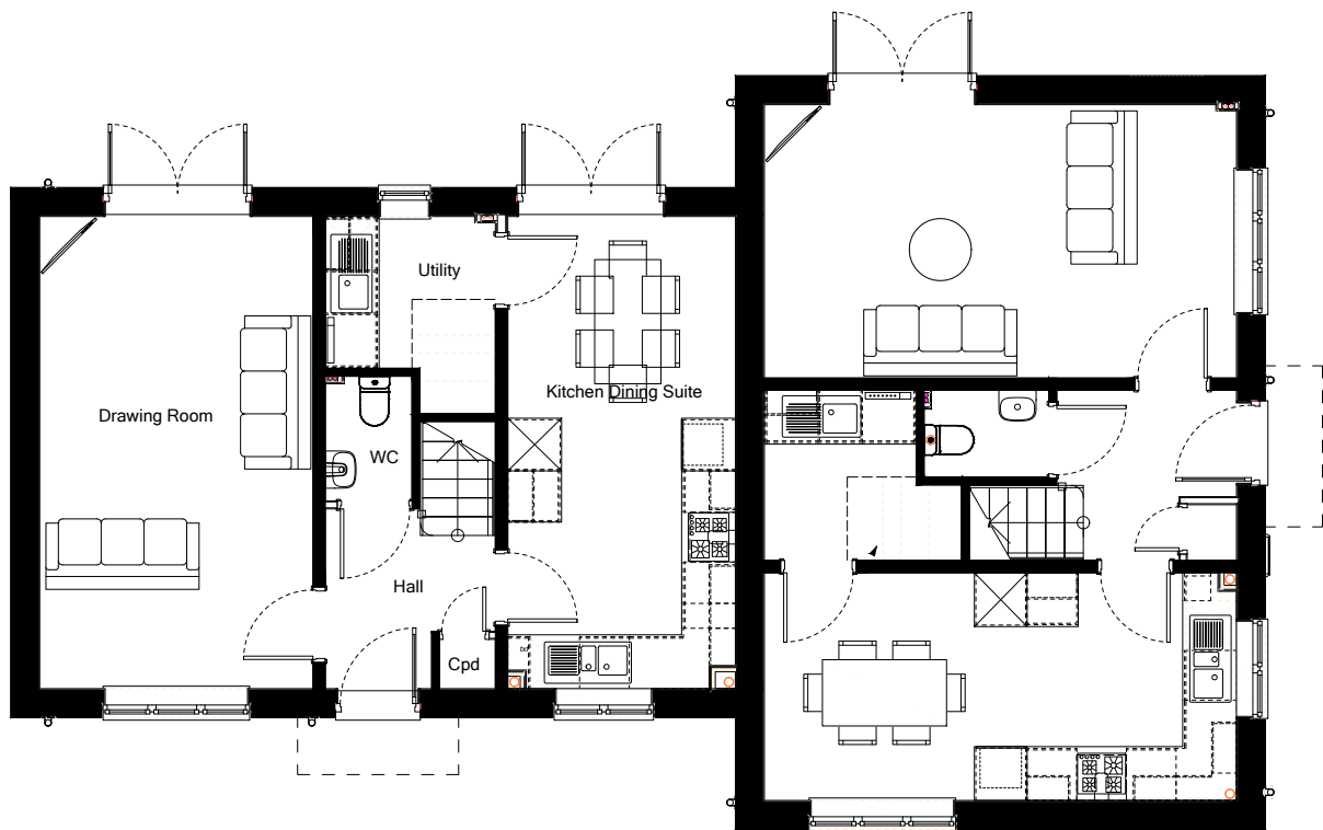
House Type K Ground Floor Plan
