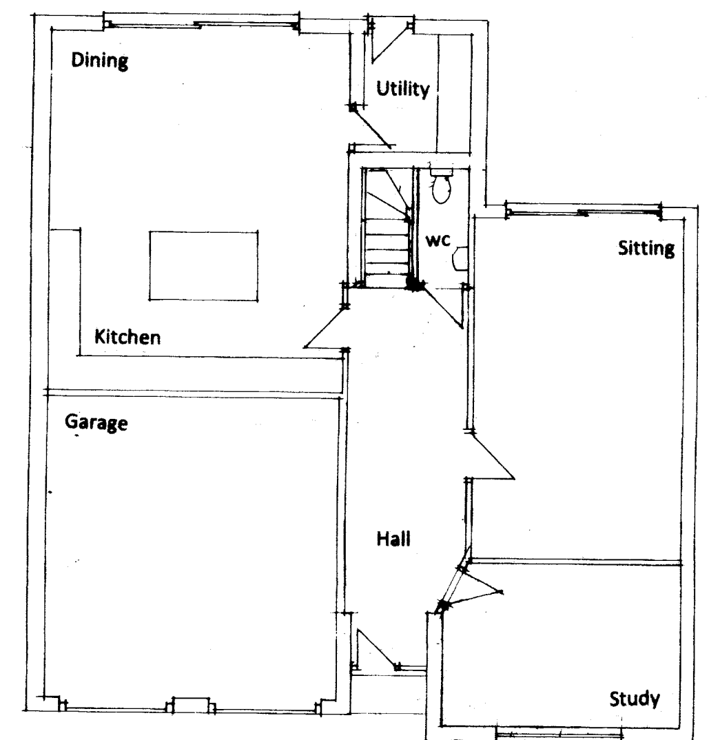
GROUND FLOOR
