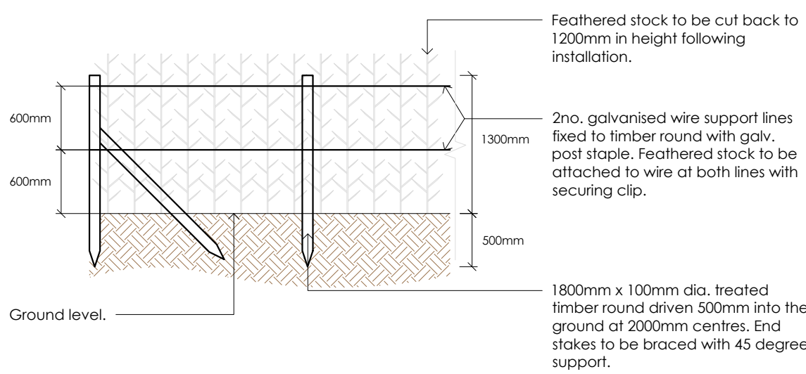
Detail 10 - Typical Feathered Stock Support Detail (N.T.S.)
