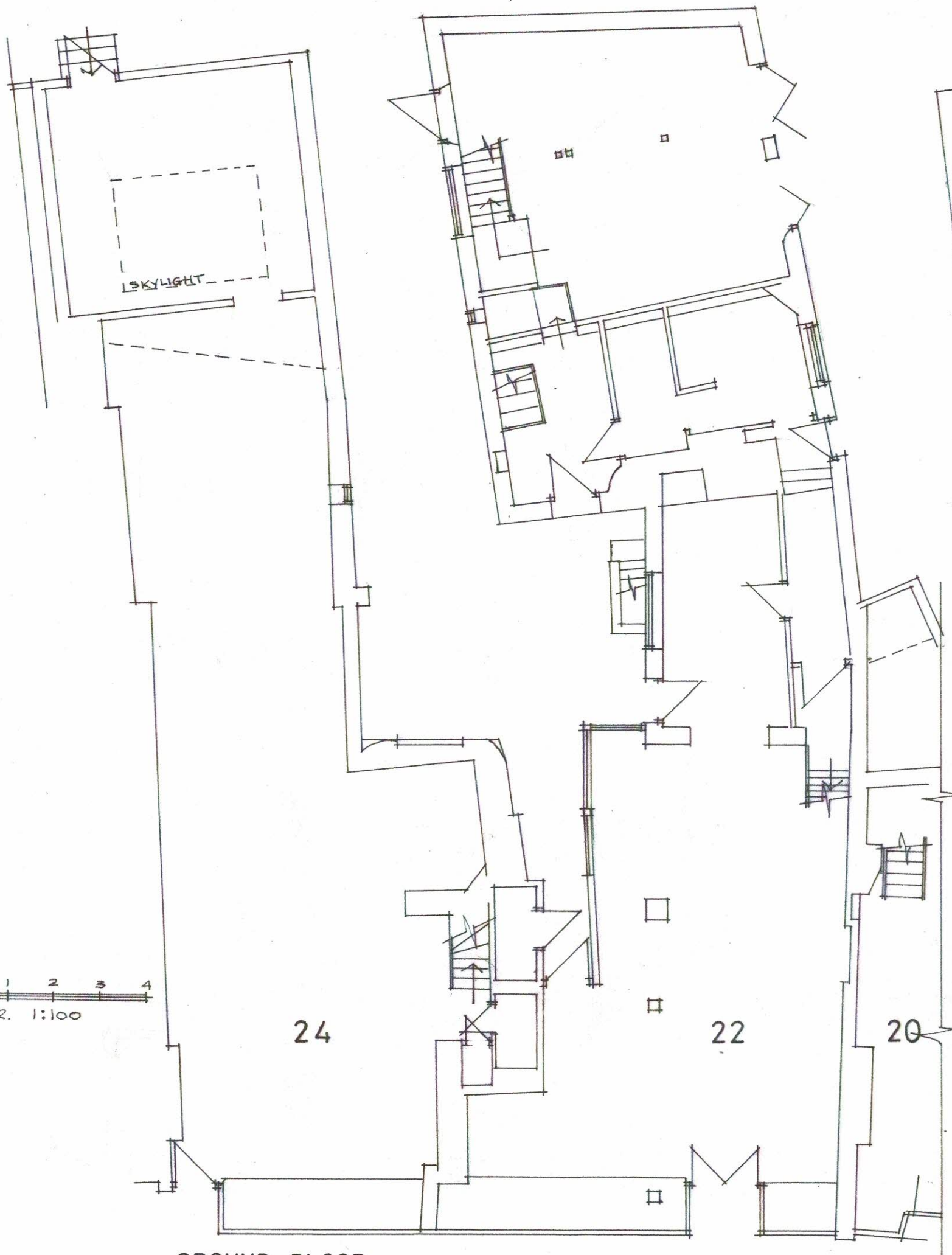
GROUND FLOOR
