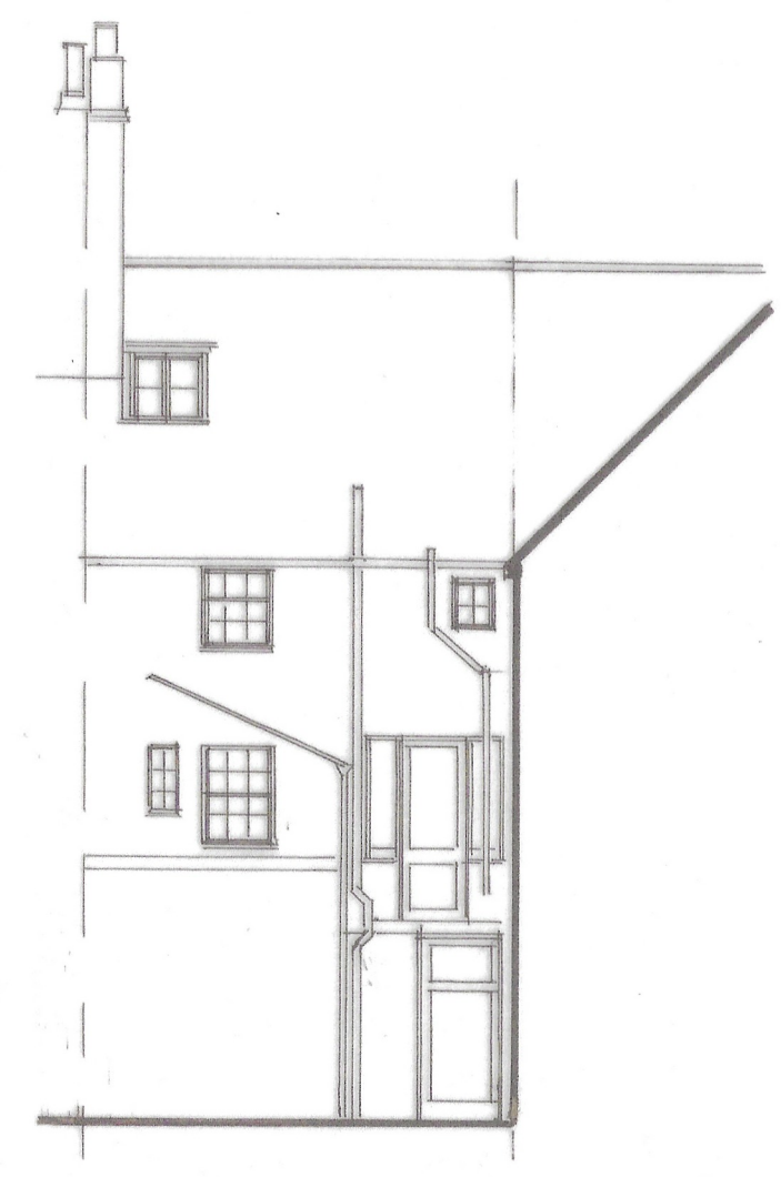
North Elevation as Existing
