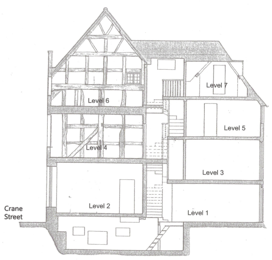
Section on A-A refer to drwg no 04525 / 2
