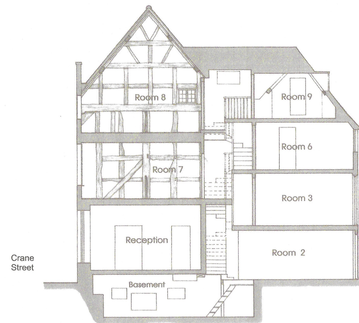
Section at A
