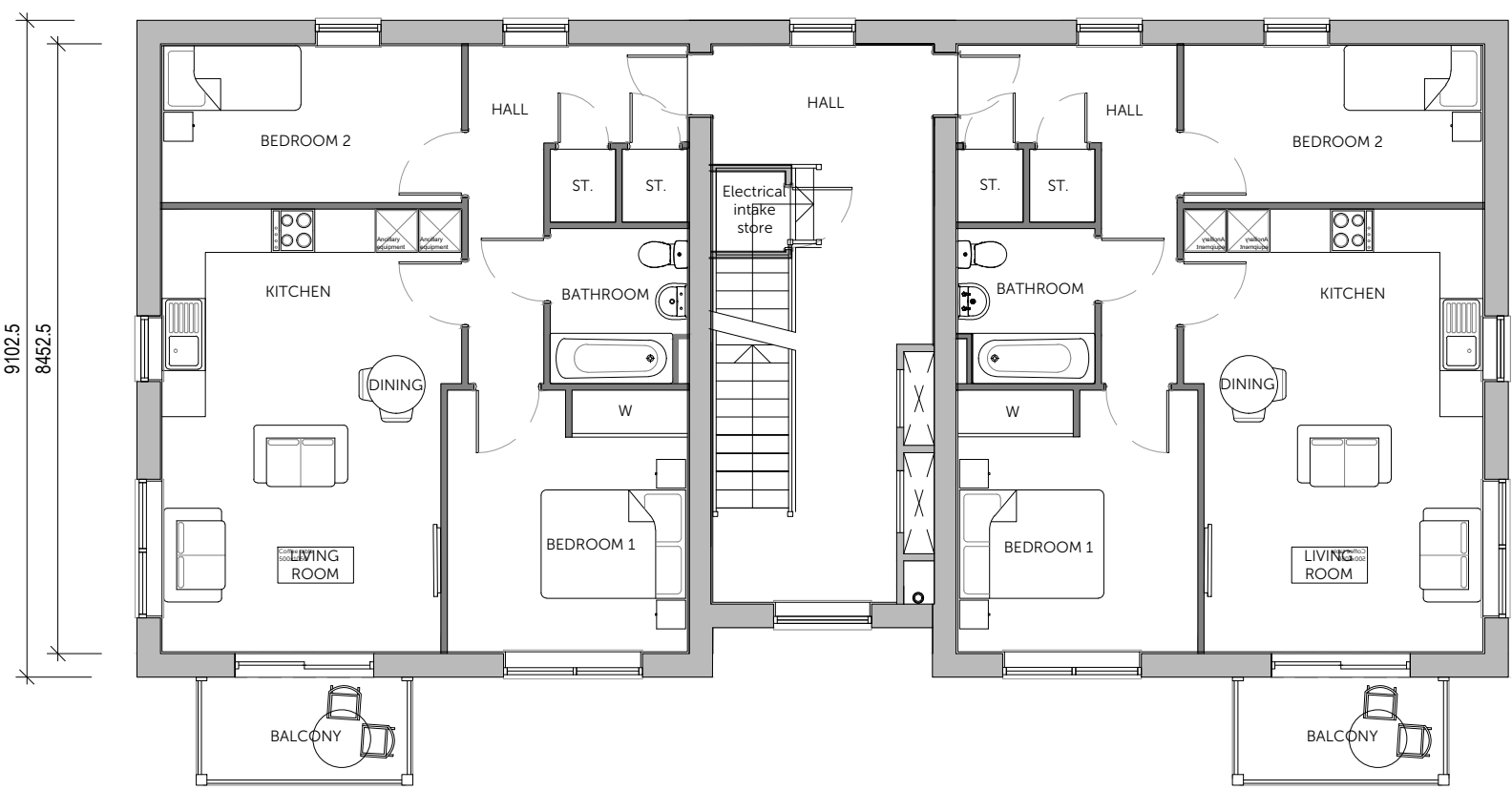
FIRST AND SECOND FLOOR PLAN
