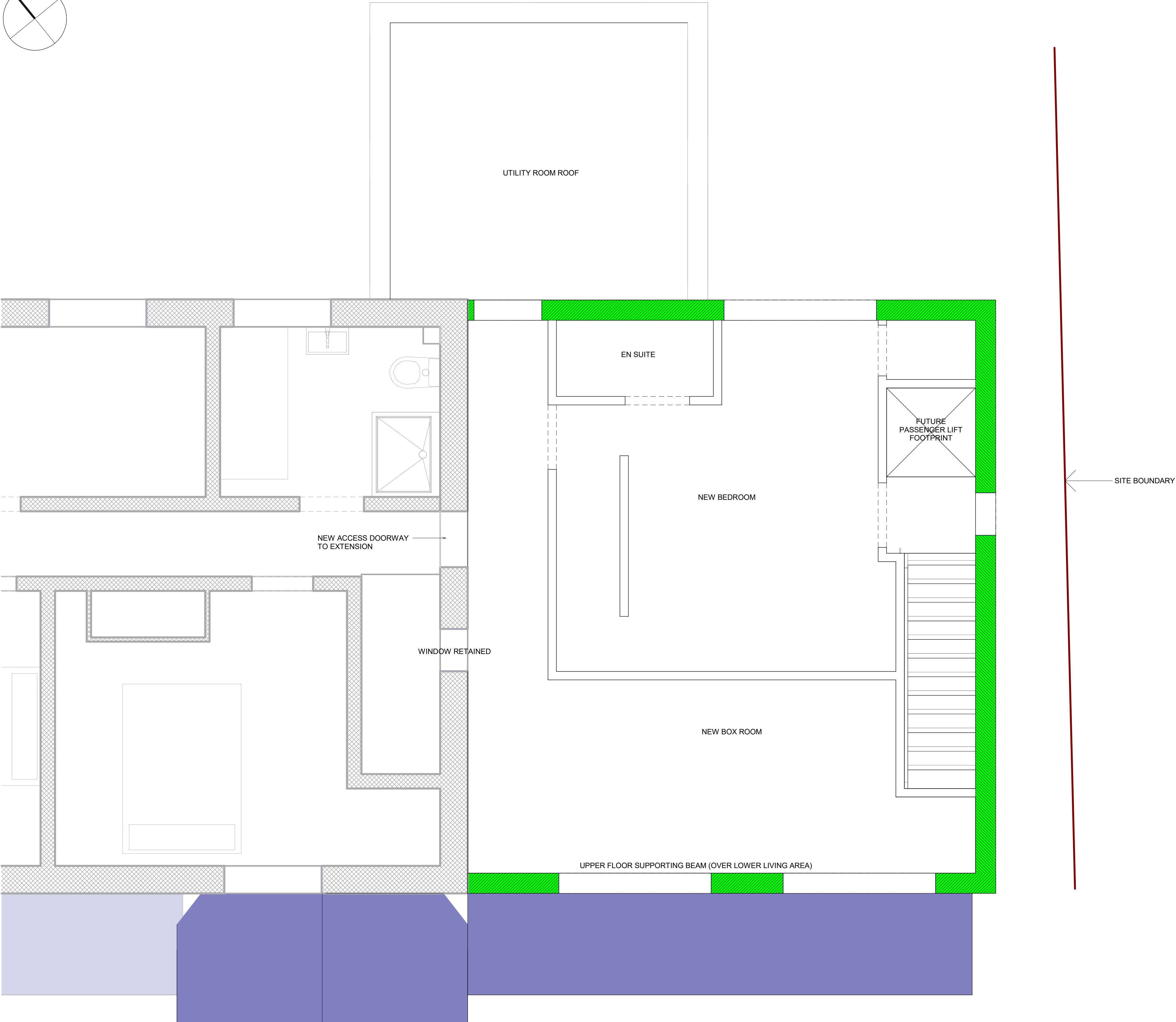
PLAN: FIRST FLOOR LEVEL Upper Floor Proposed Plan Scale: 1 : 25
