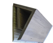
2 x Soffit mounted timber bat box 300L x 140D x 250H. Google Image 5
