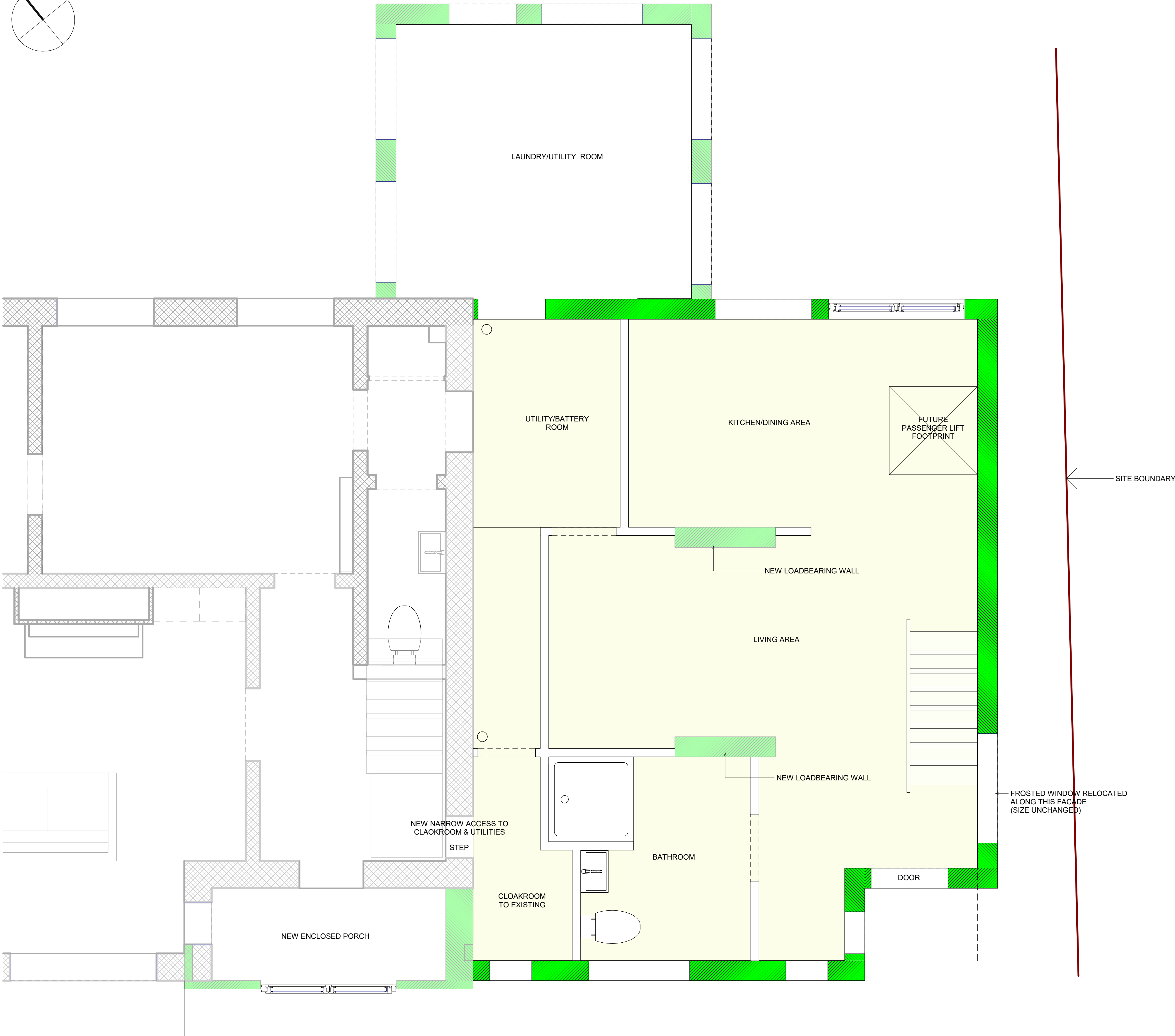
PLAN: GROUND FLOOR LEVEL Ground Floor Proposed Plan Scale: 1 : 25
