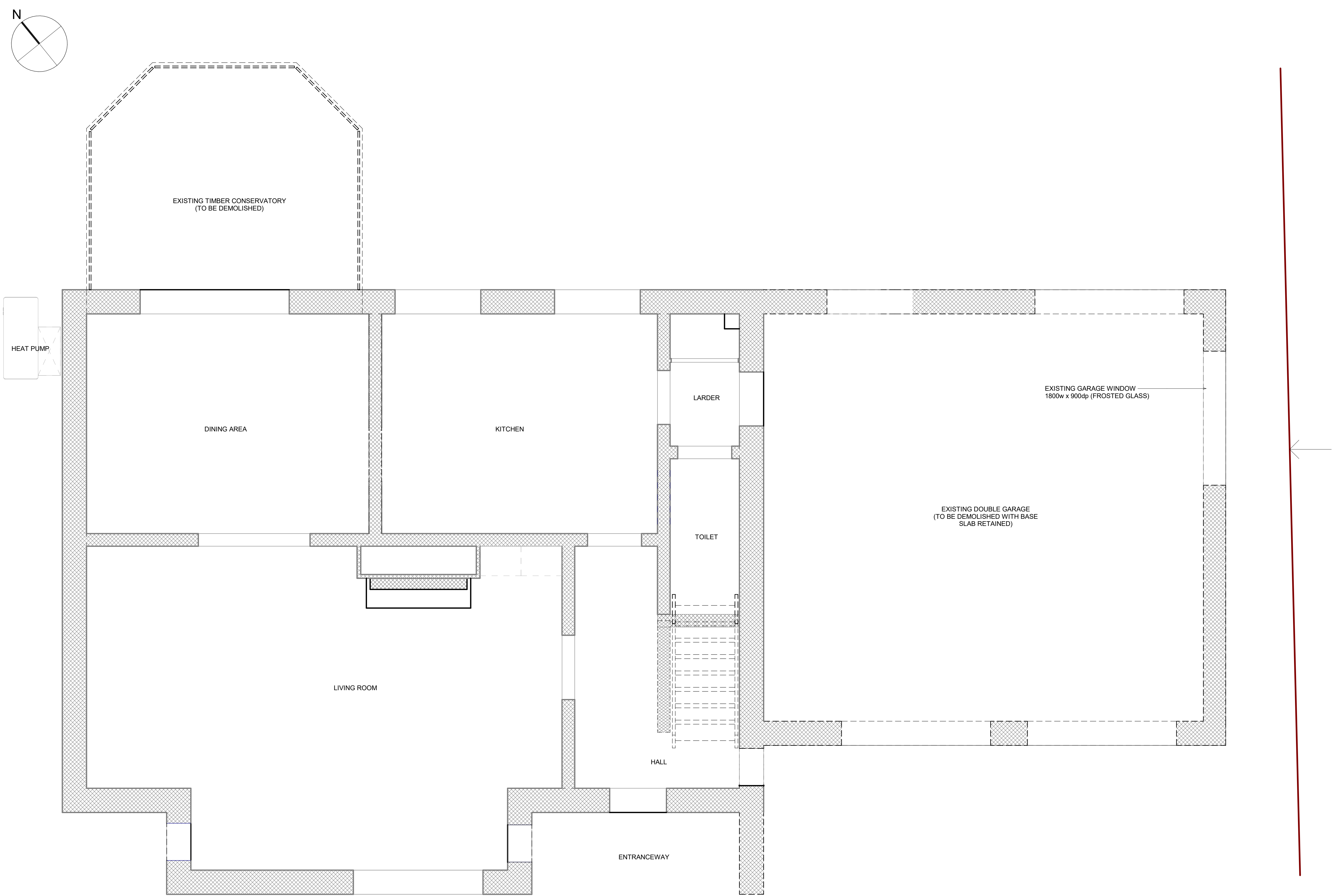
PLAN: GROUND FLOOR LEVEL Ground Floor Existing Plan Scale: 1 : 25
