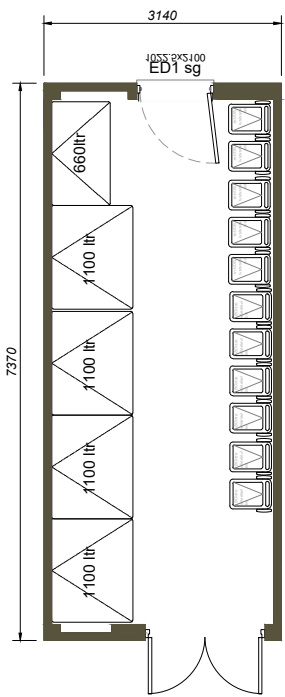
Plan
