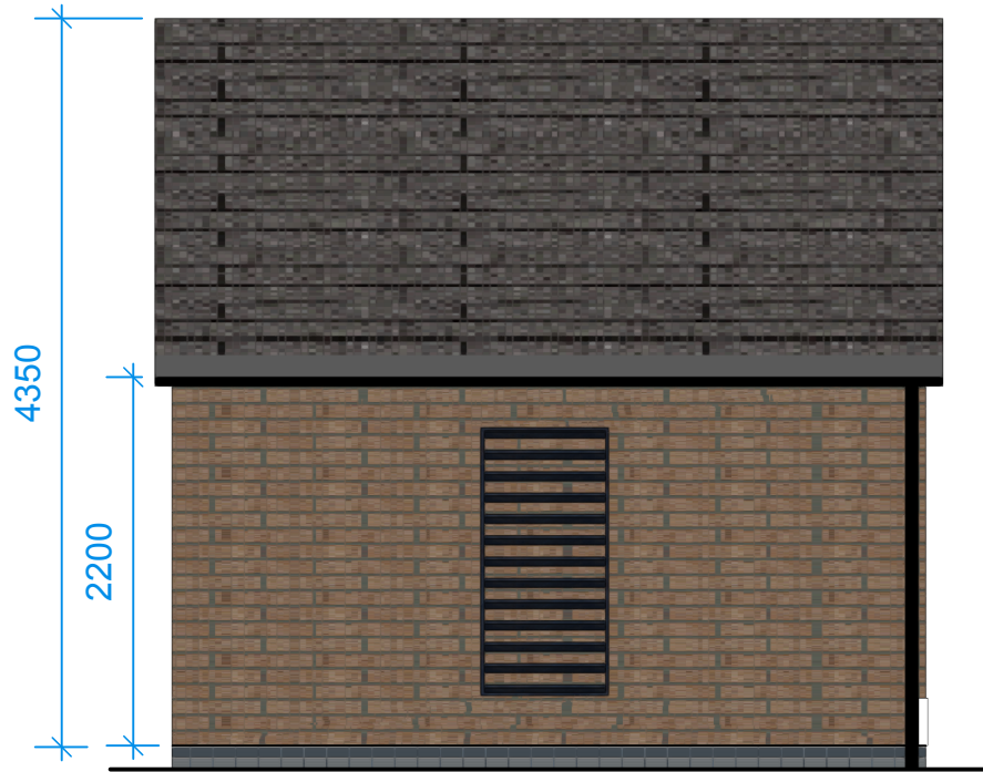
01 Bin Store - Side Elevation
