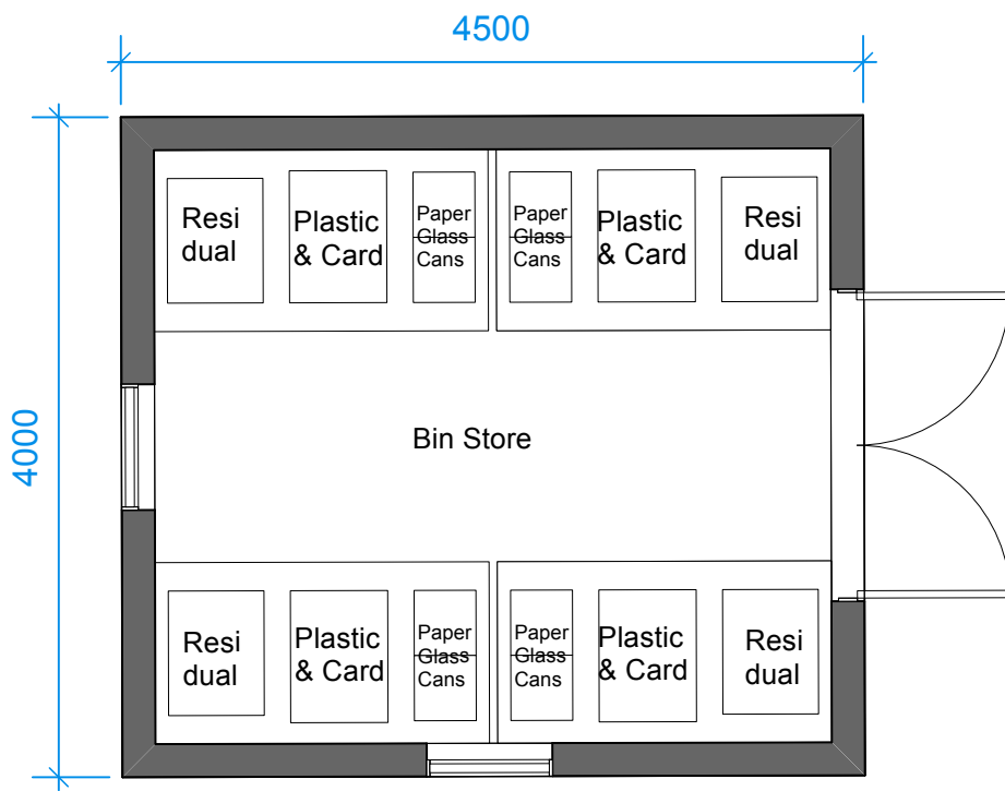
02 Bin Store - Floor Plan
