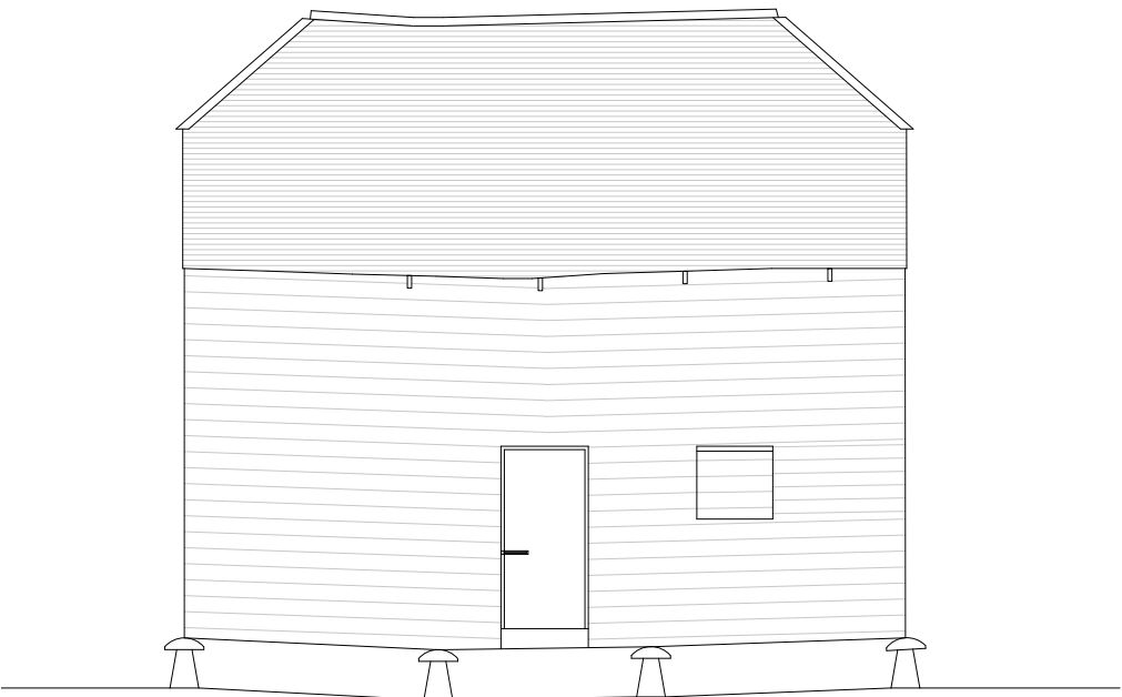
WEST ELEVATION - EXISTING AND PROPOSED
