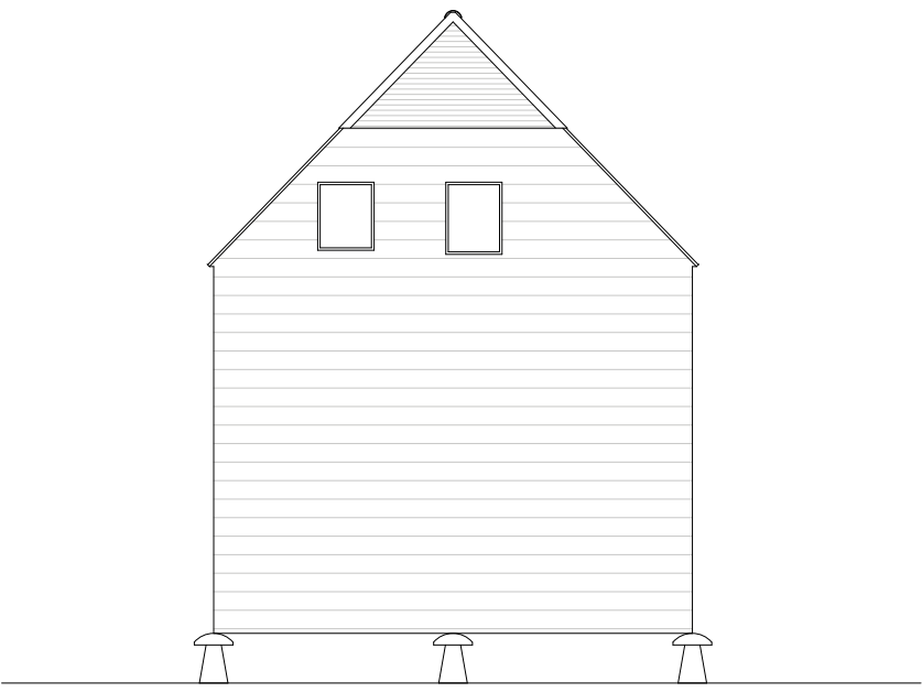
SOUTH ELEVATION - EXISTING AND PROPOSED
