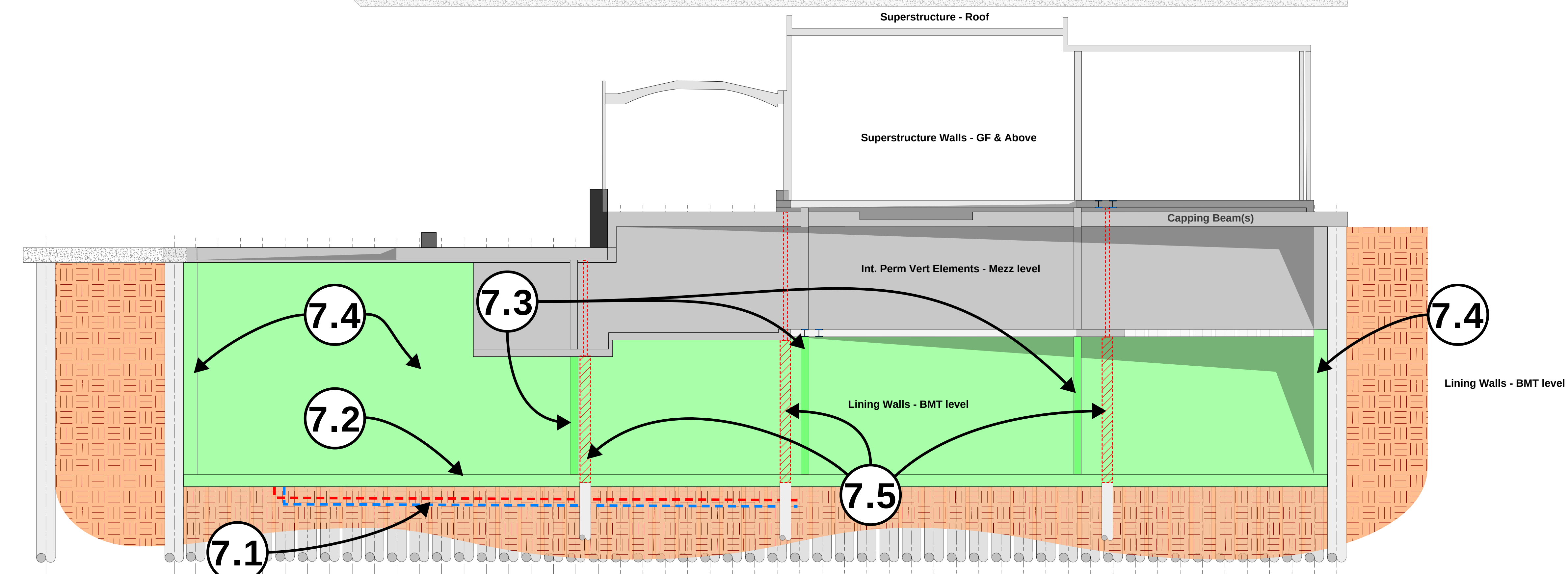
SECTION
