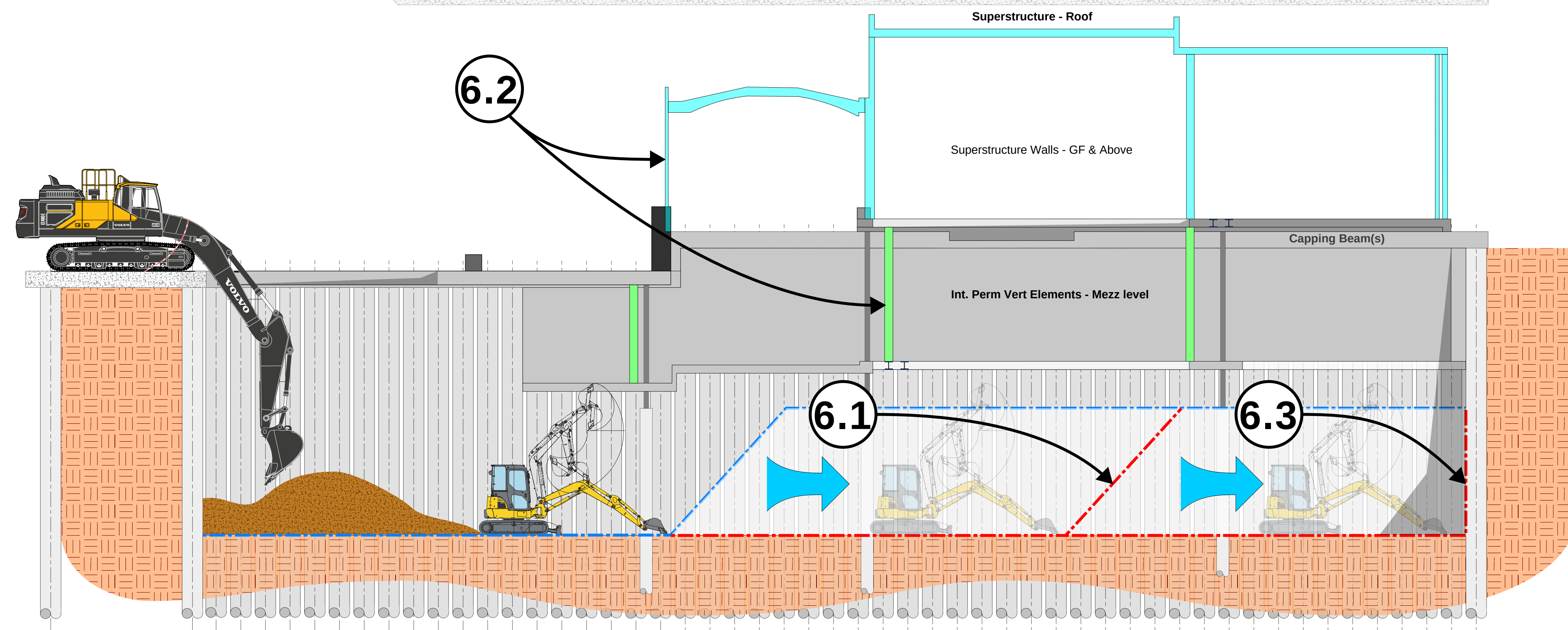
SECTION
