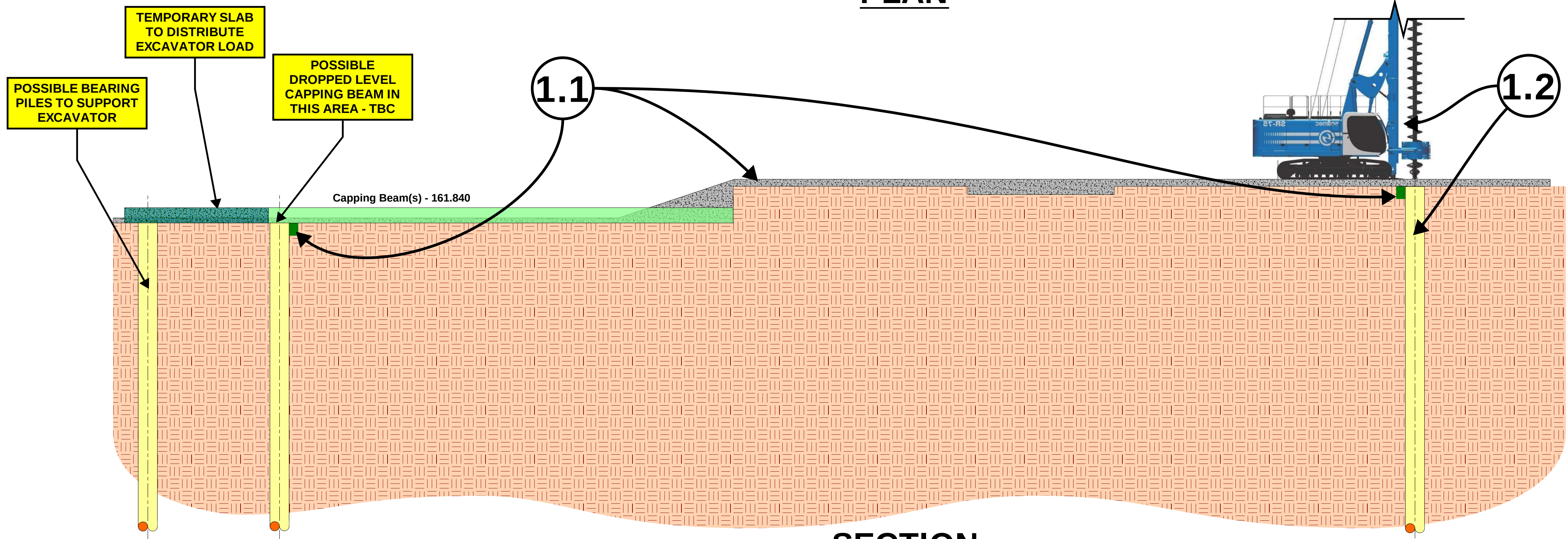
SECTION
