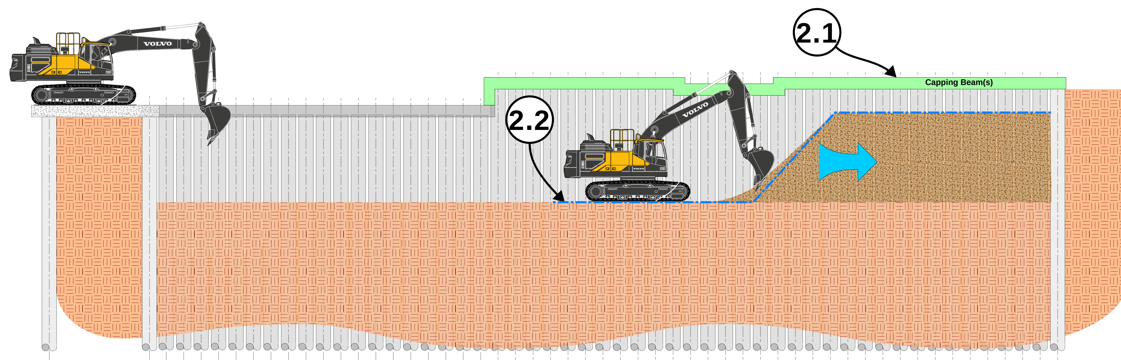
SECTION
