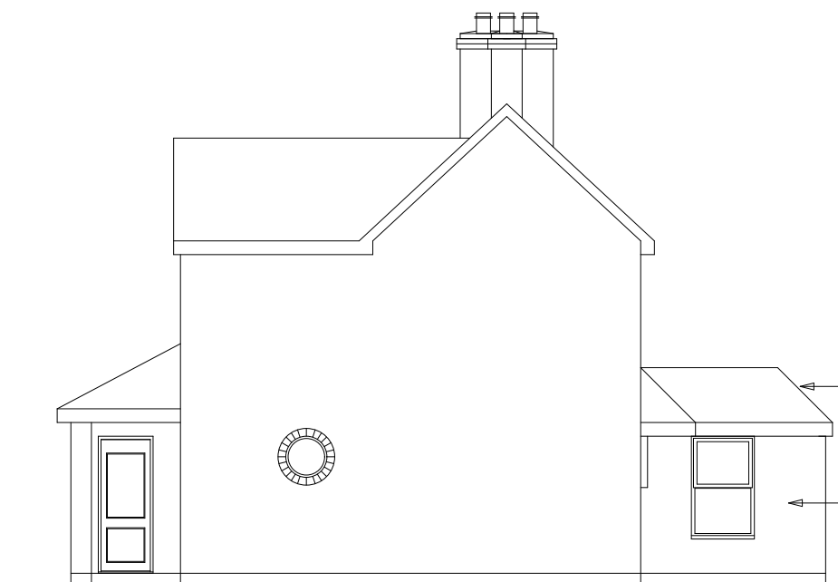
Proposed Side
