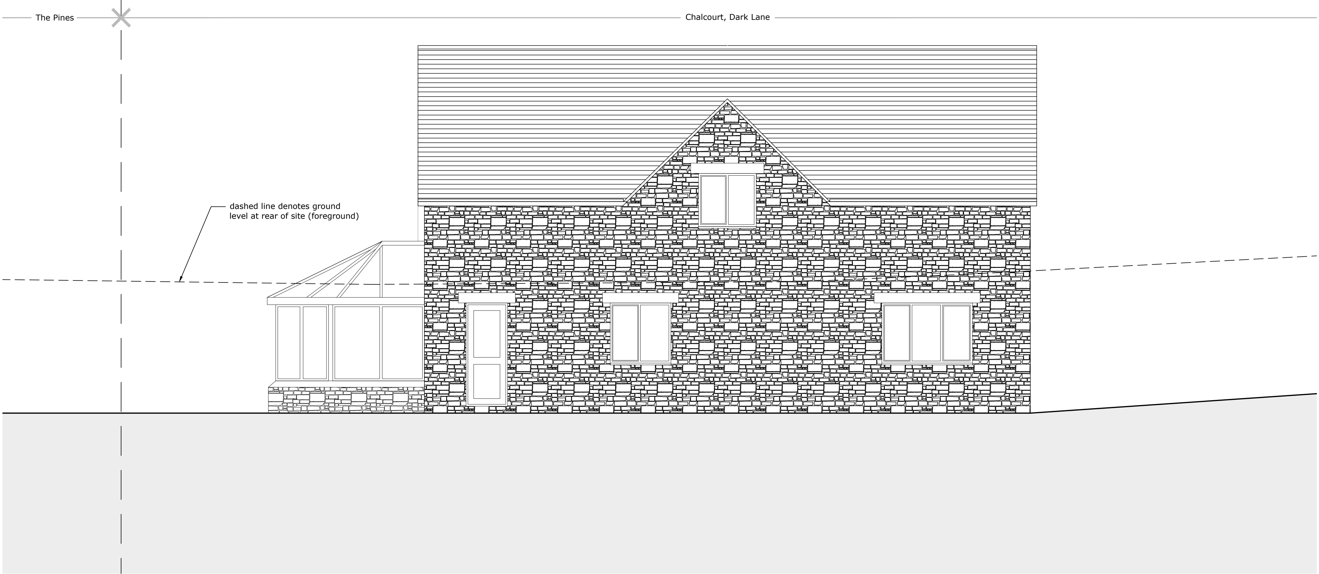
rear elevation (north facing) as existing 1:50
