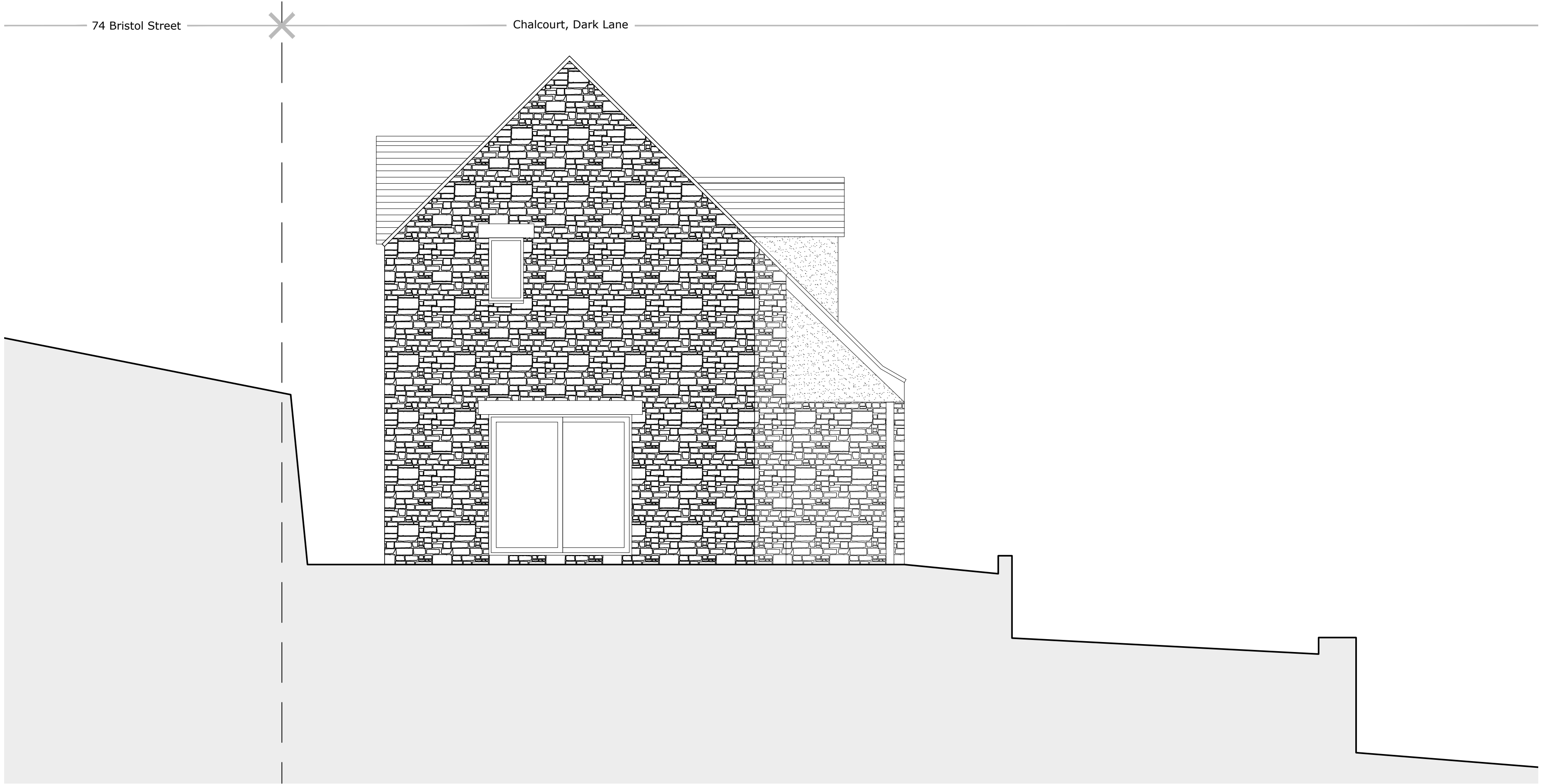
side elevation (west facing) as proposed 1:50
