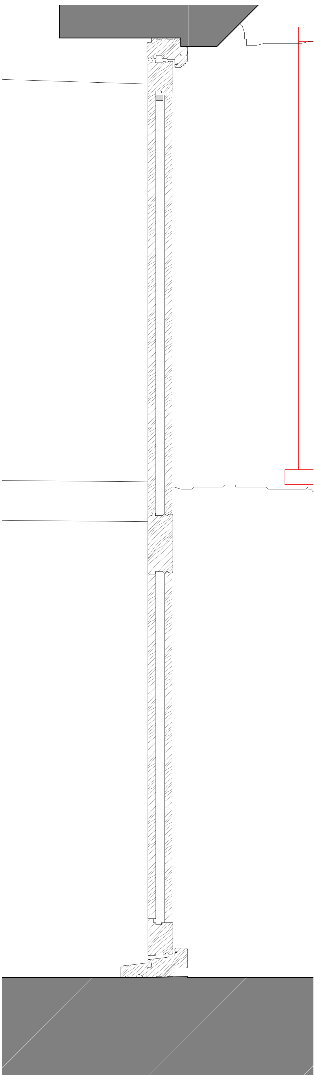
Vertical Section - Front Door
