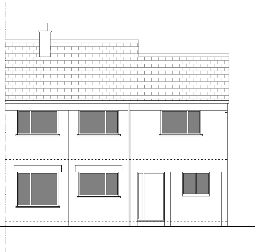
FRONT (NW) ELEVATION - scale 1:100
