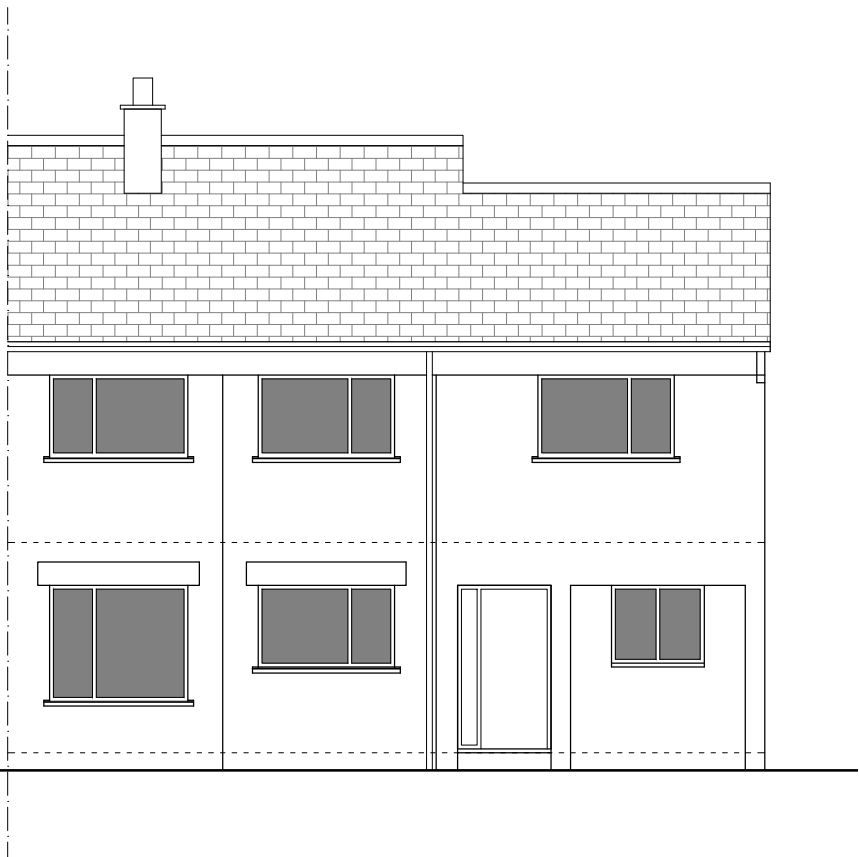
FRONT (NW) ELEVATION - scale 1:100
