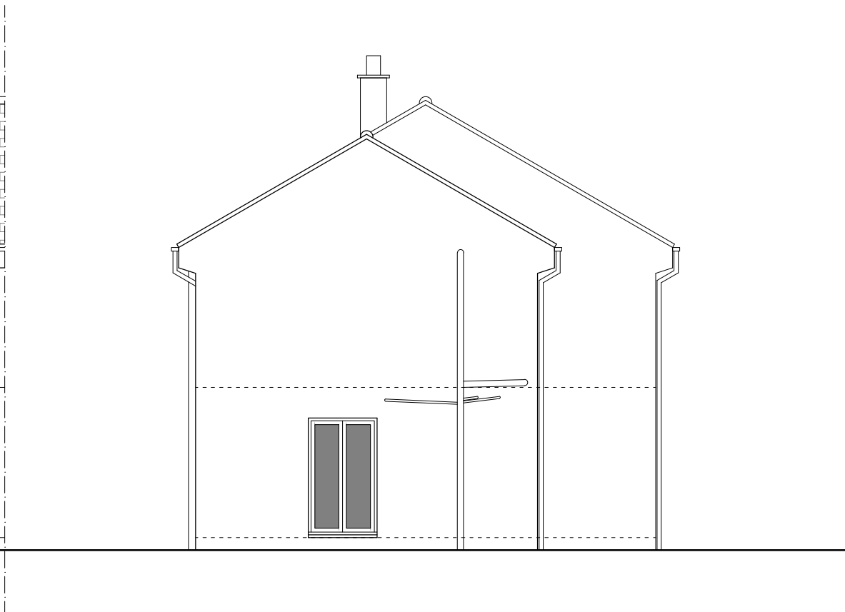
SIDE (SW) ELEVATION - scale 1:100
