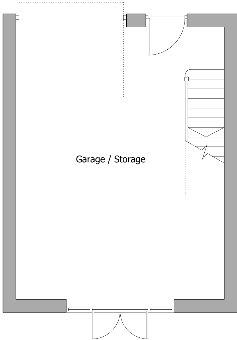
Ground Floor Plan 1:50 @ A3
