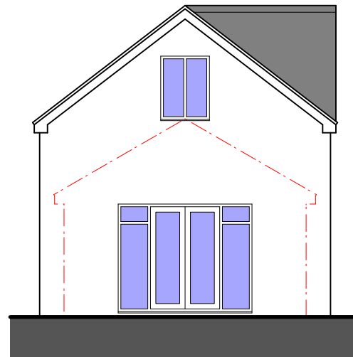
Proposed Rear Elevation 1:100 @ A3
