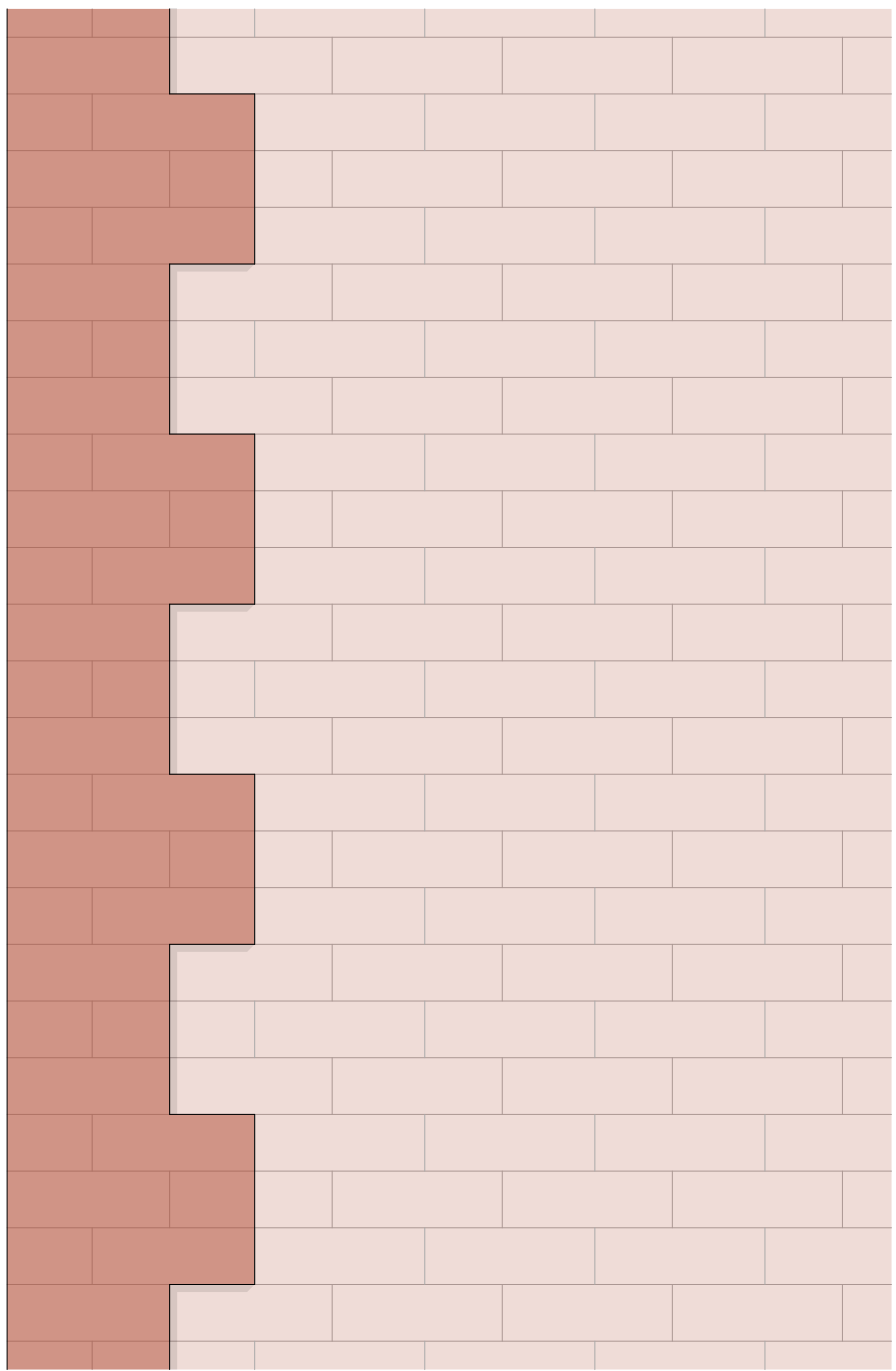
DET 03 Brick Quoin Detail 1:10
