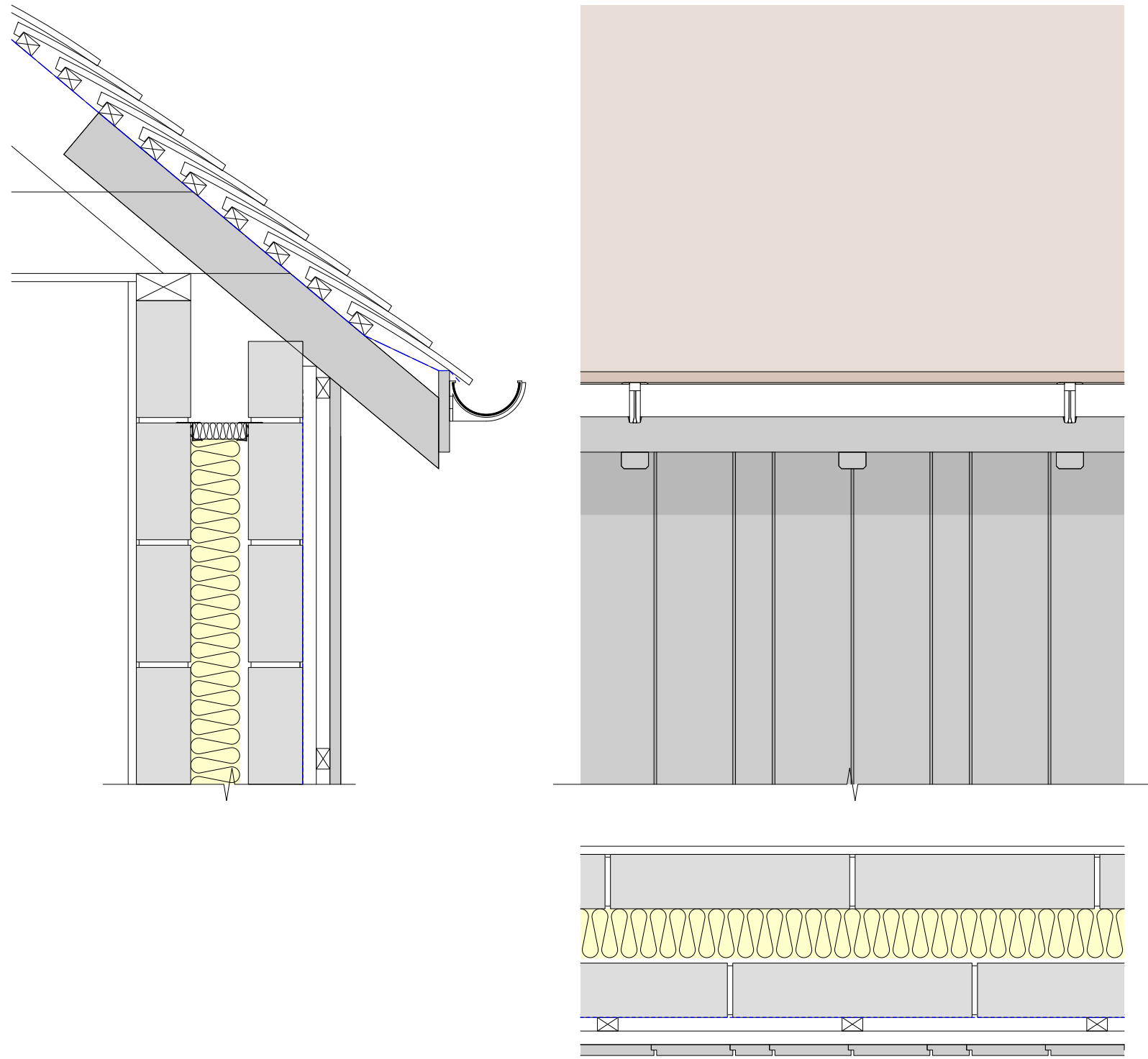
DET 01 Eaves Detail 01 1:10
