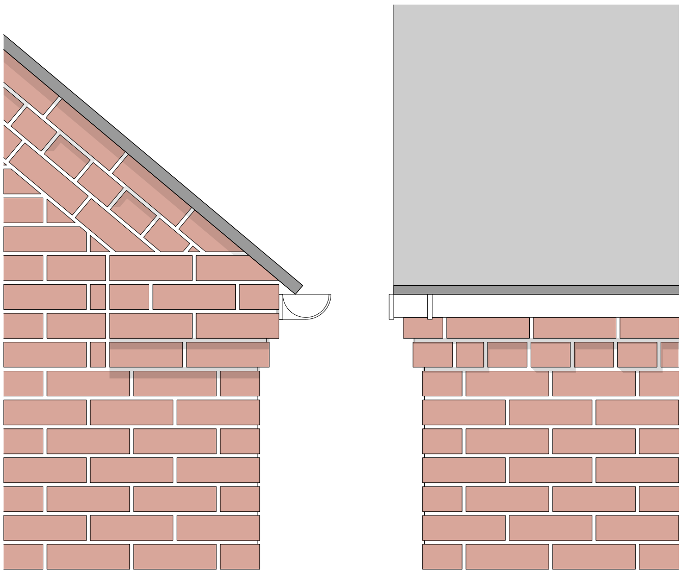
DET 02 Eaves Detail 02 1:10
