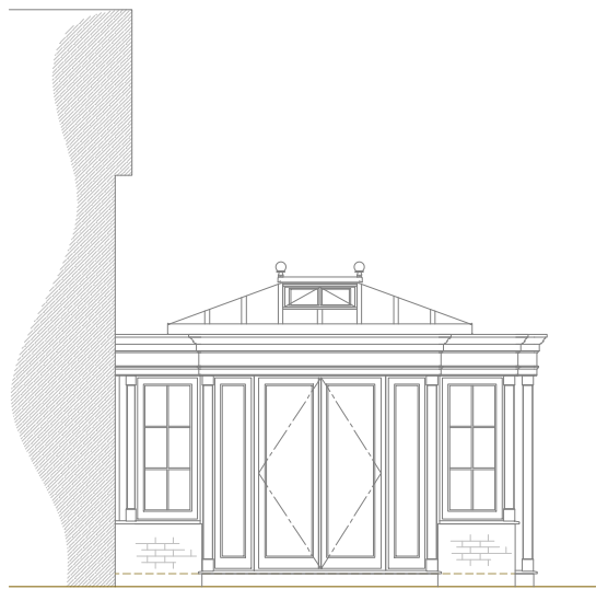
PROPOSED NORTH - EAST ELEVATION (Orangery) Scale 1:100
