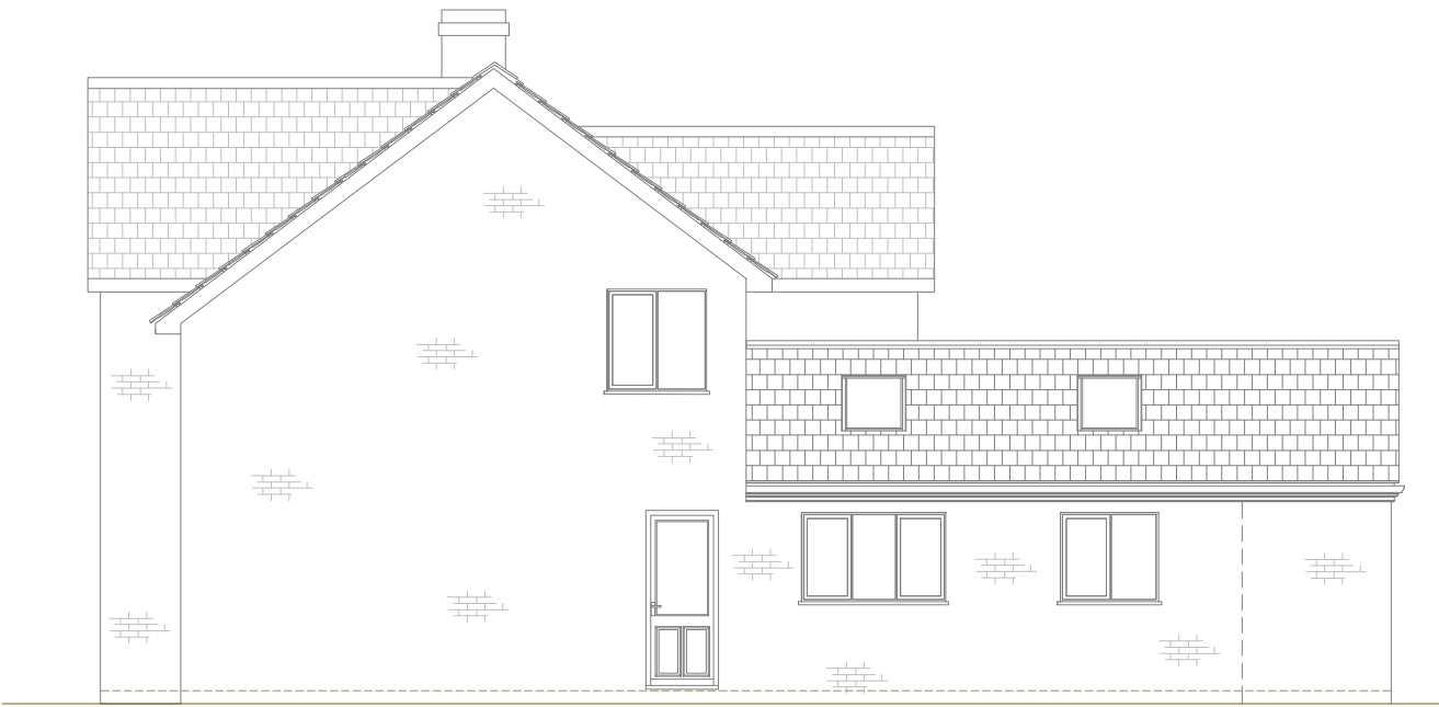
PROPOSED NORTH - EAST ELEVATION Scale 1:100
