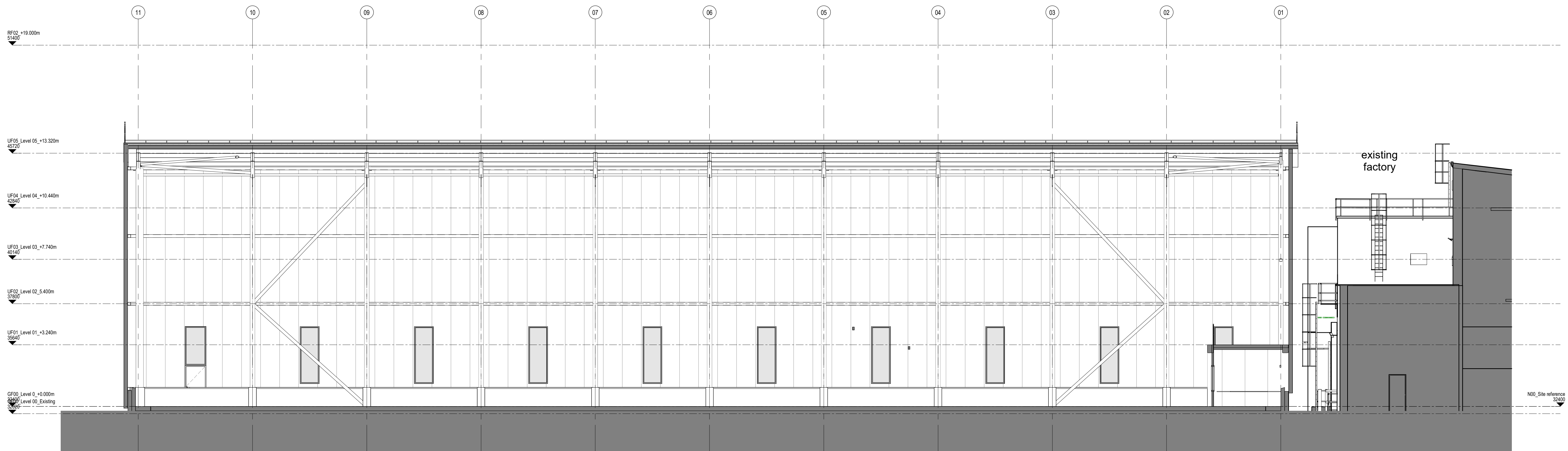
Proposed Section J-J 1 : 100
