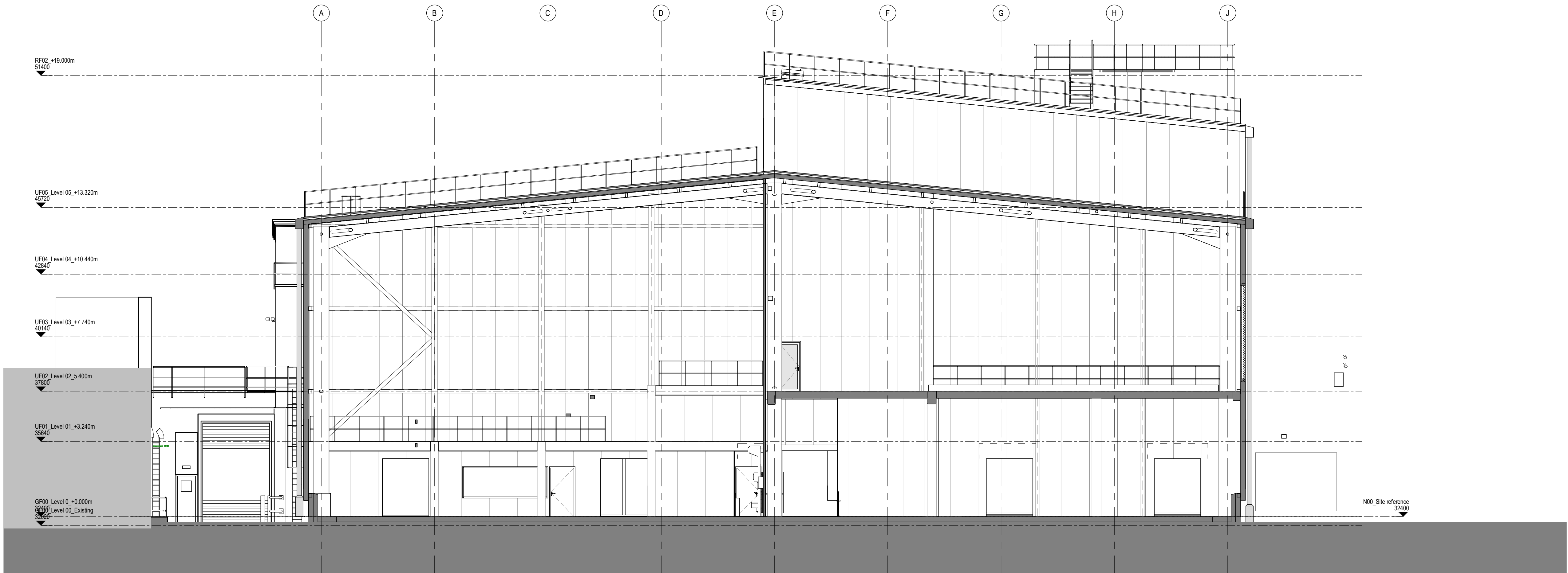
Proposed Section D-D 1 : 100
