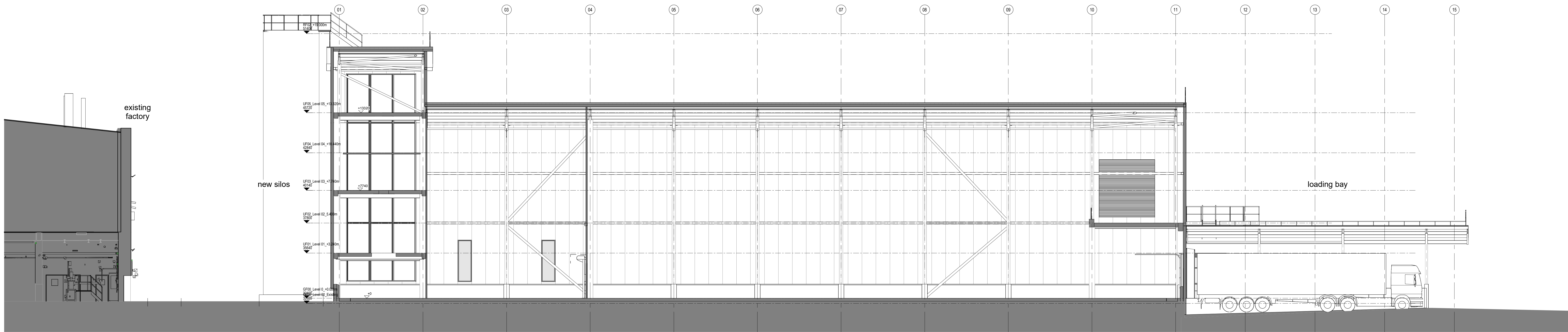
Proposed Section A-A 1 : 100
