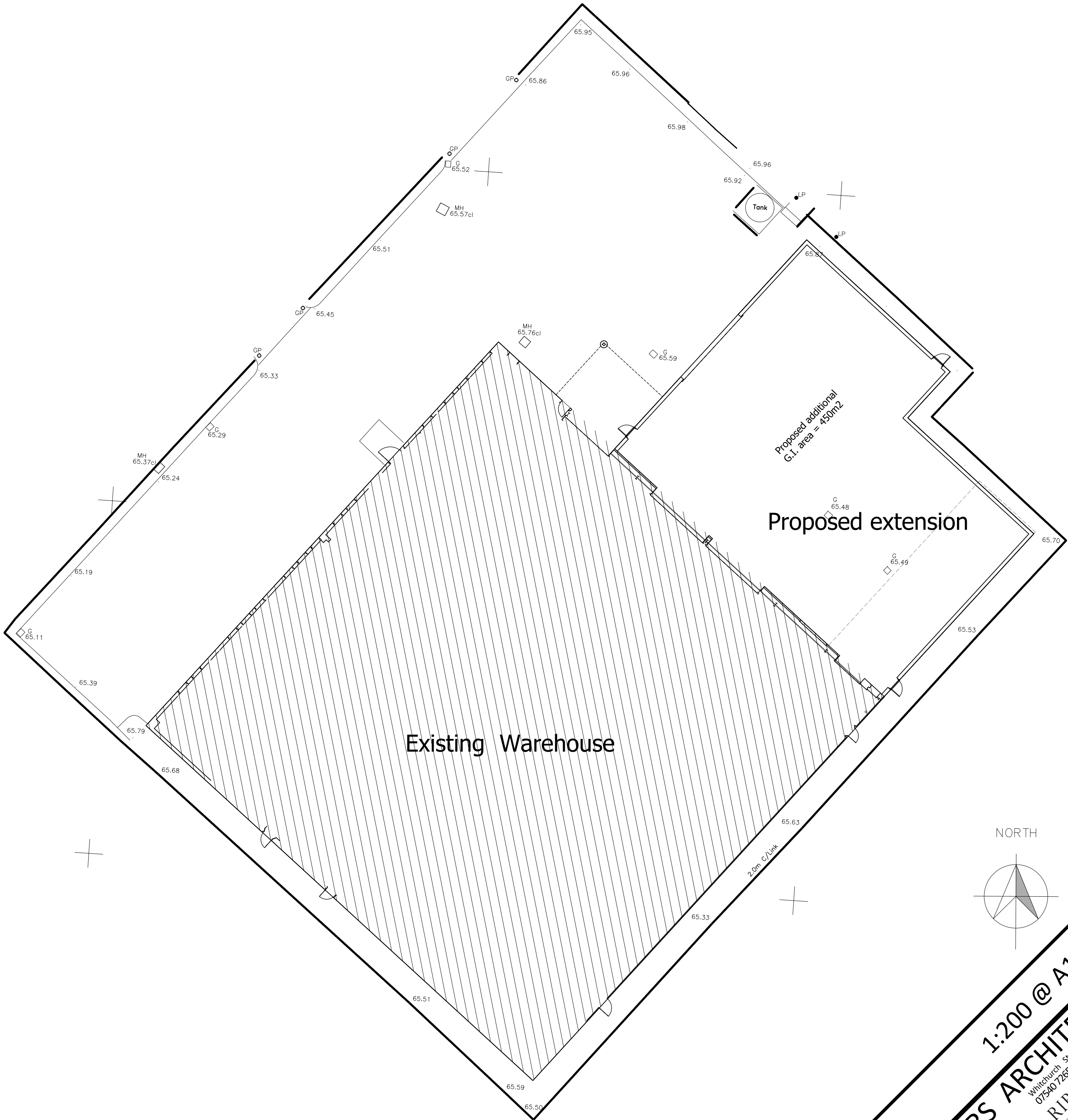
PROPOSED FLOOR PLAN
