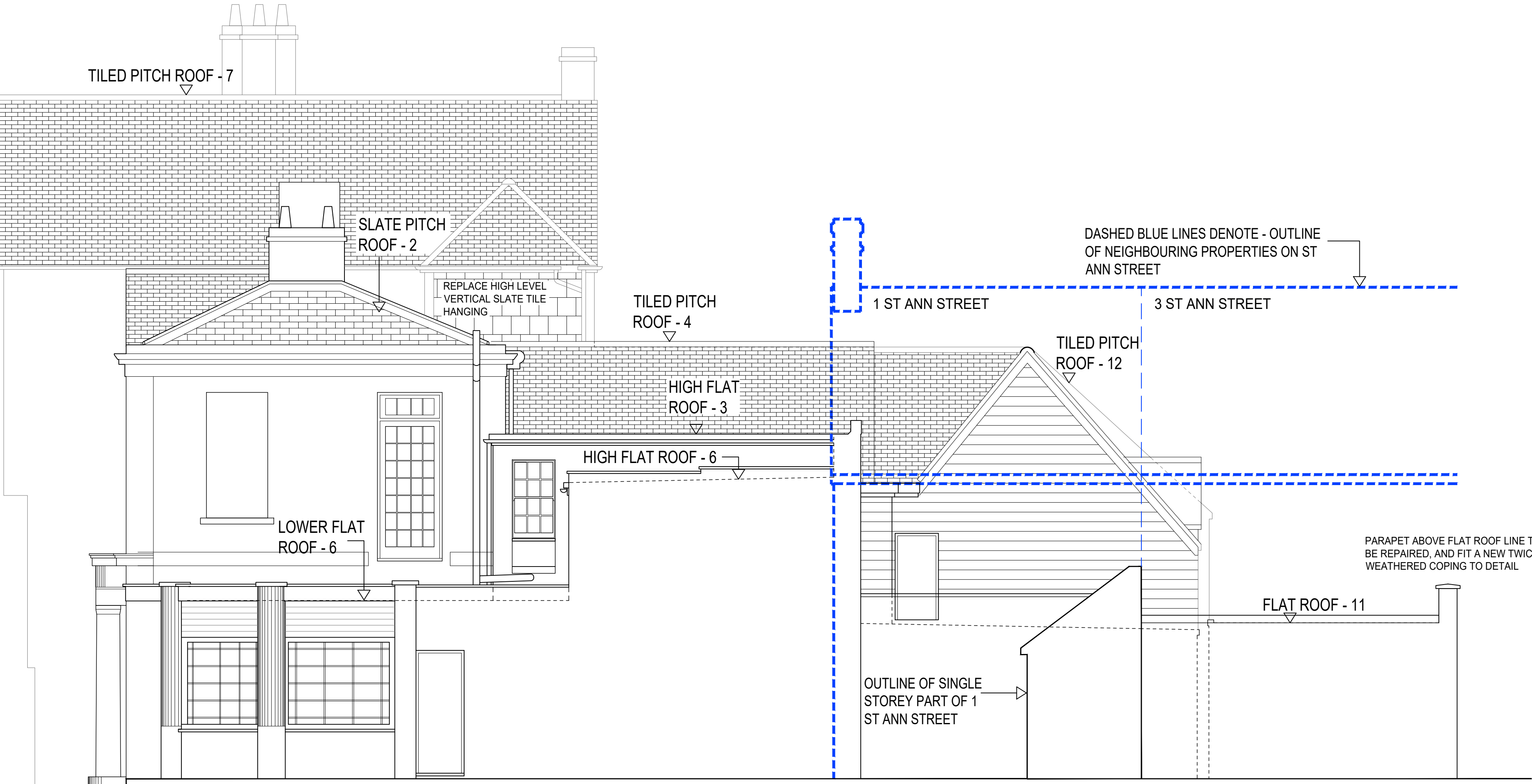
PROPOSED ST ANN STREET (SOUTH) ELEVATION @ SCALE 1:50
