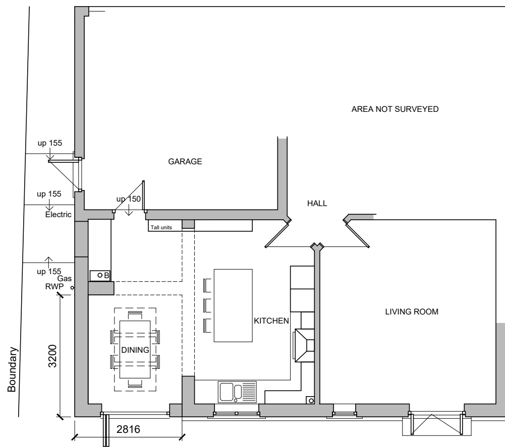
GROUND FLOOR PROPOSED PART FLOOR PLAN scale 1:100
