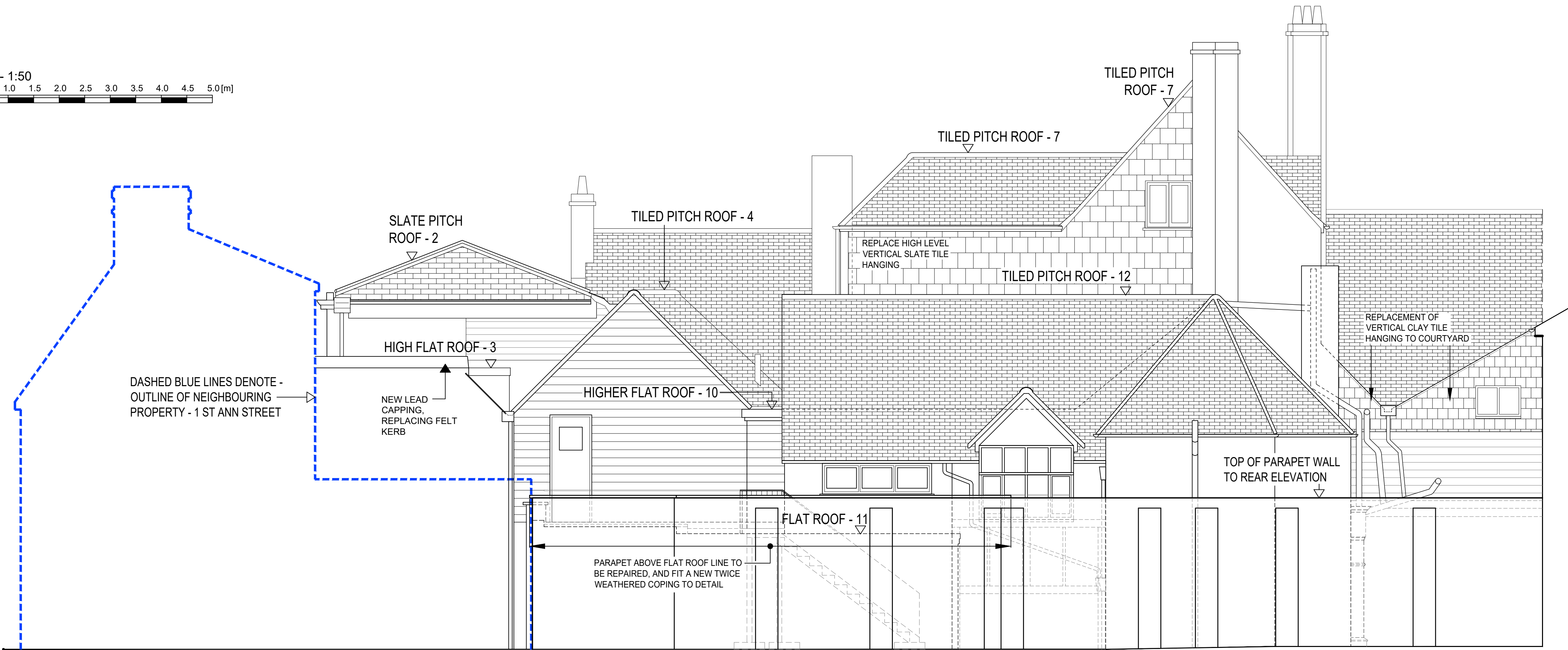
PROPOSED REAR (EAST) ELEVATION, (VIEWED FROM WITHIN CAR PARK)
