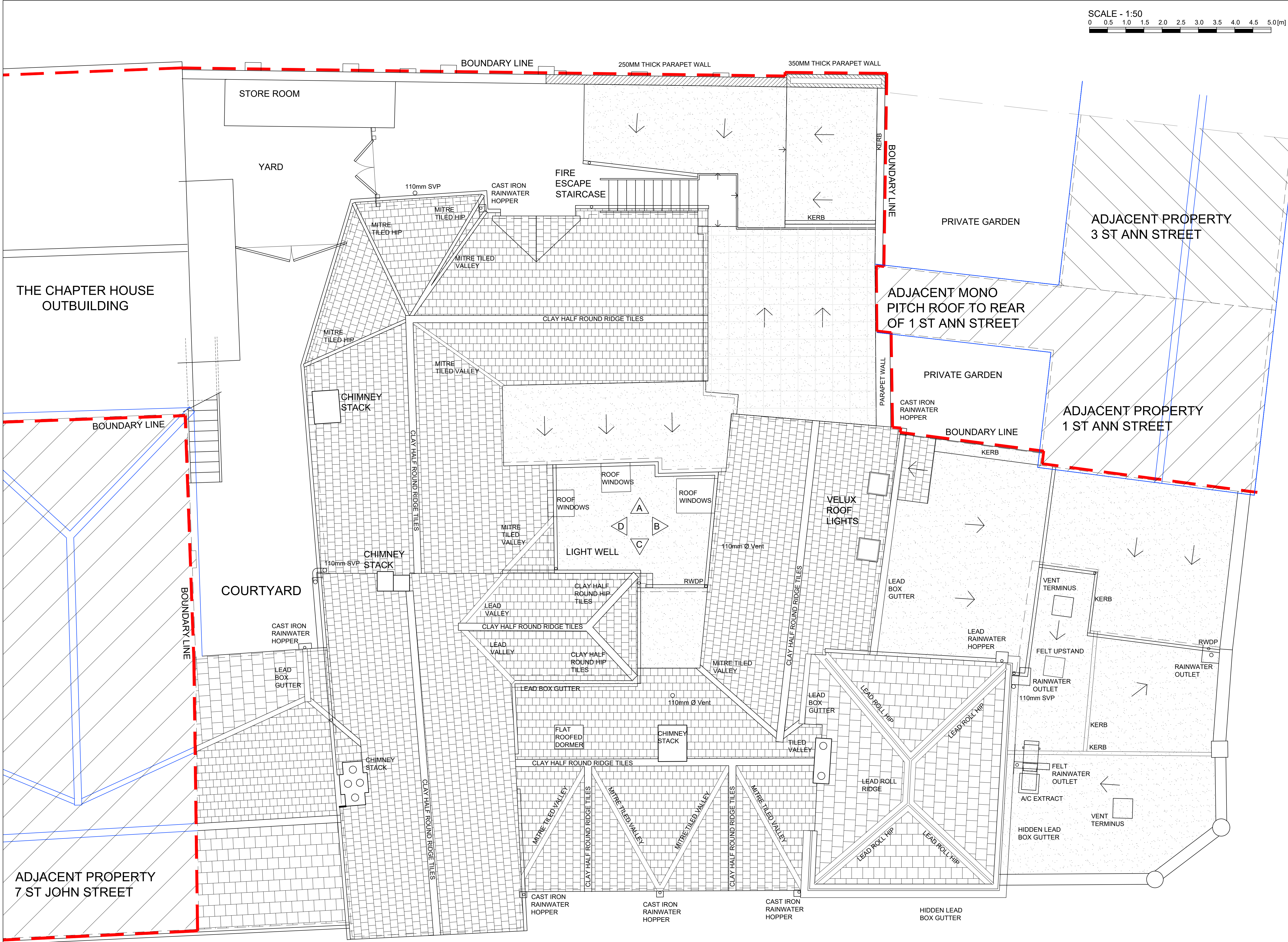
EXISTING ROOF LAYOUT @ SCALE 1:50
