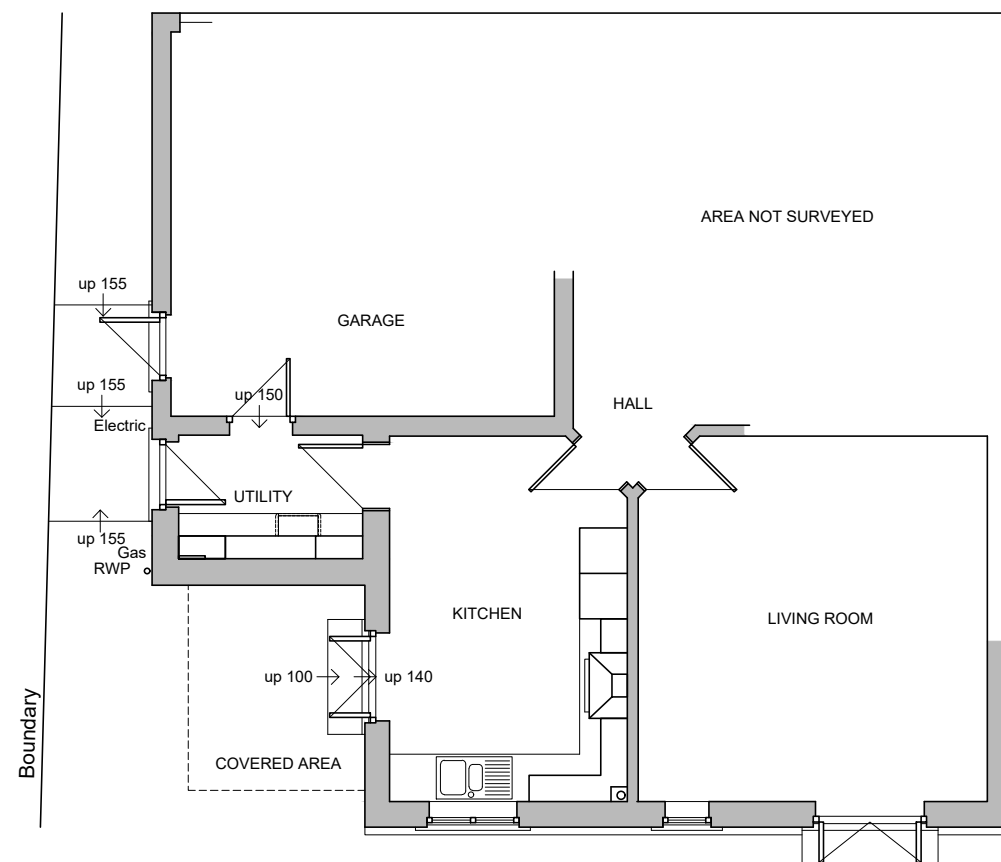
GROUND FLOOR EXISTING PART FLOOR PLAN scale 1:100
