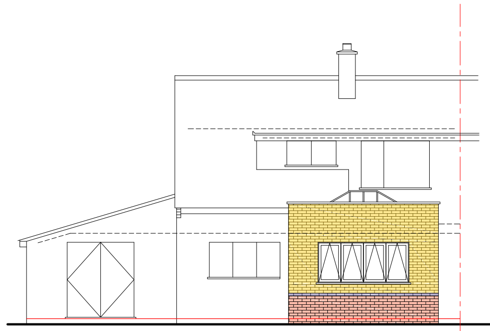
PROPOSED REAR (EAST) ELEVATION
