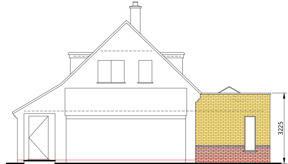
PROPOSED SIDE (SOUTH) ELEVATION
