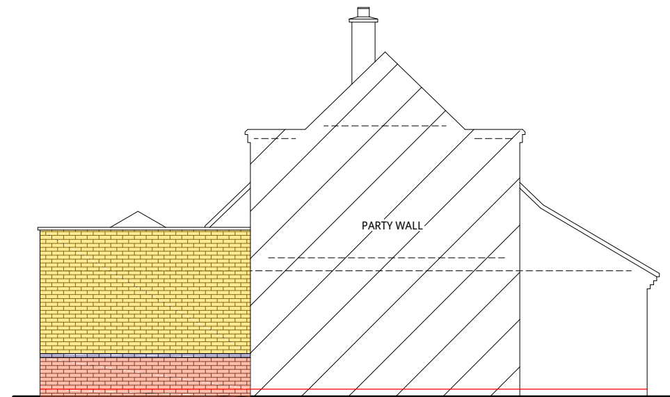
PROPOSED SIDE (NORTH) ELEVATION
