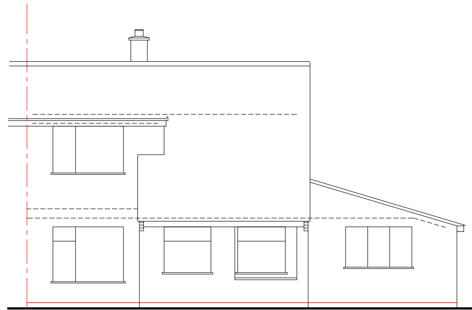
EXISTING FRONT (WEST) ELEVATION
