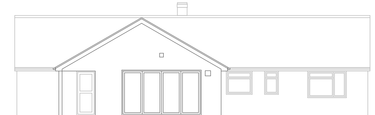
REAR ELEVATION
