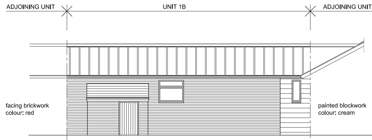
REAR ELEVATION
