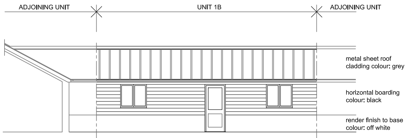
FRONT ELEVATION
