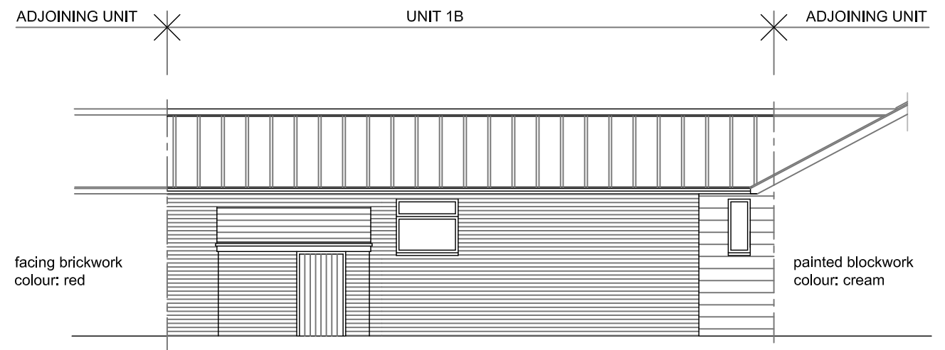
REAR ELEVATION
