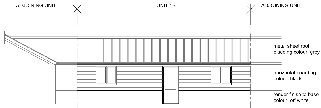
FRONT ELEVATION
