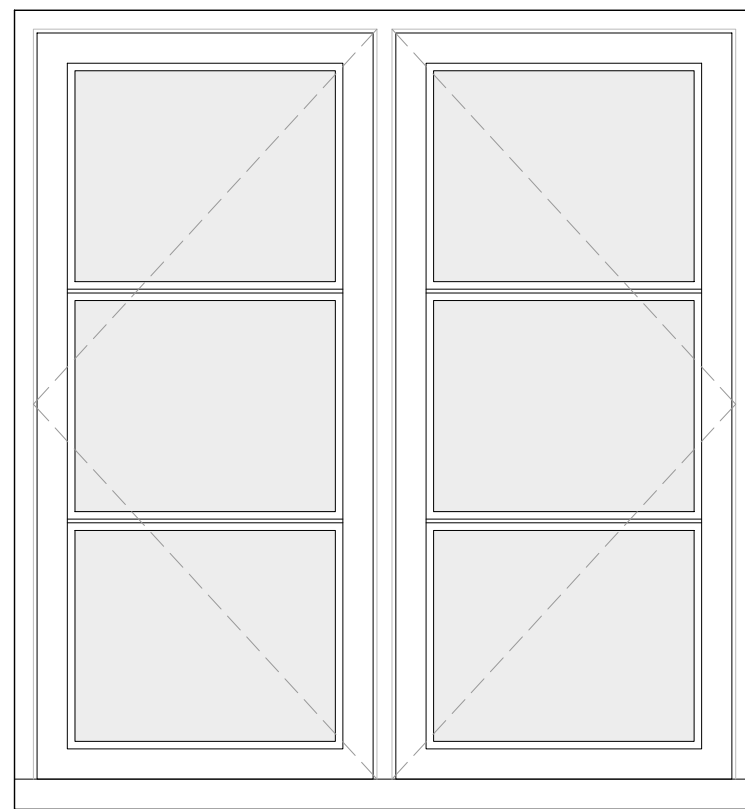
DINING ROOM (SW ele) EXTERNAL ELEVATION (980w x 1050h) 1:10
