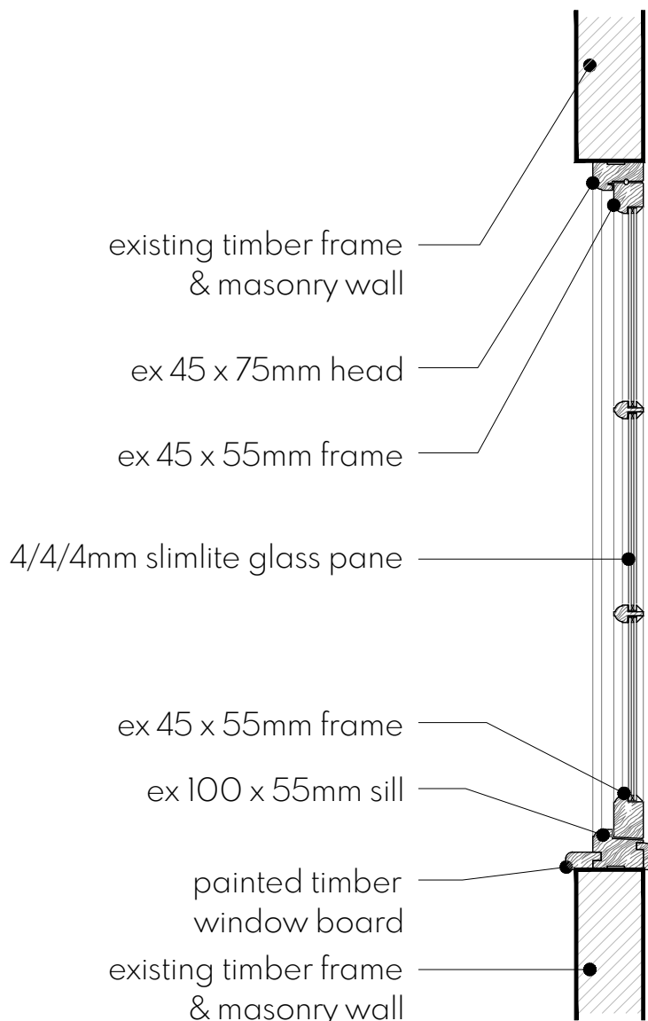
VERTICAL SECTION 1:10
