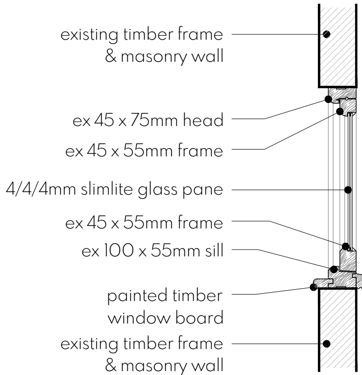
VERTICAL SECTION 1:10
