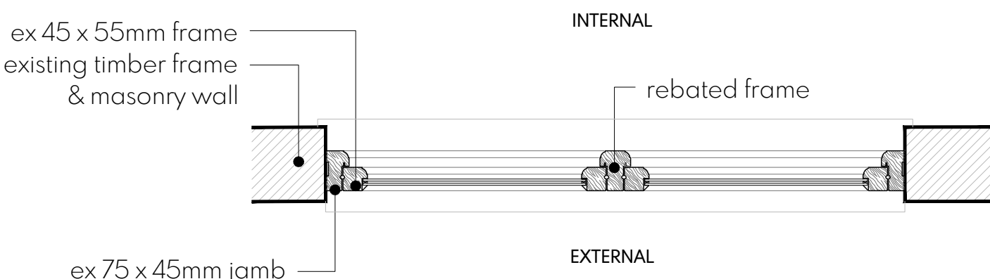
HORIZONTAL SECTION 1:10
