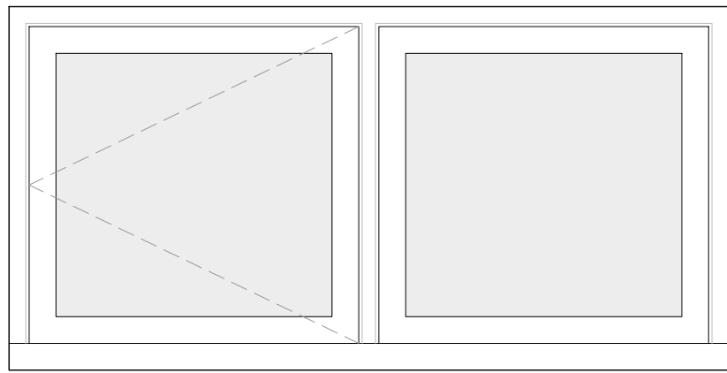
UTILITY WINDOWS (SW ele LHS) EXTERNAL ELEVATION (1075w x 545h) 1:10
