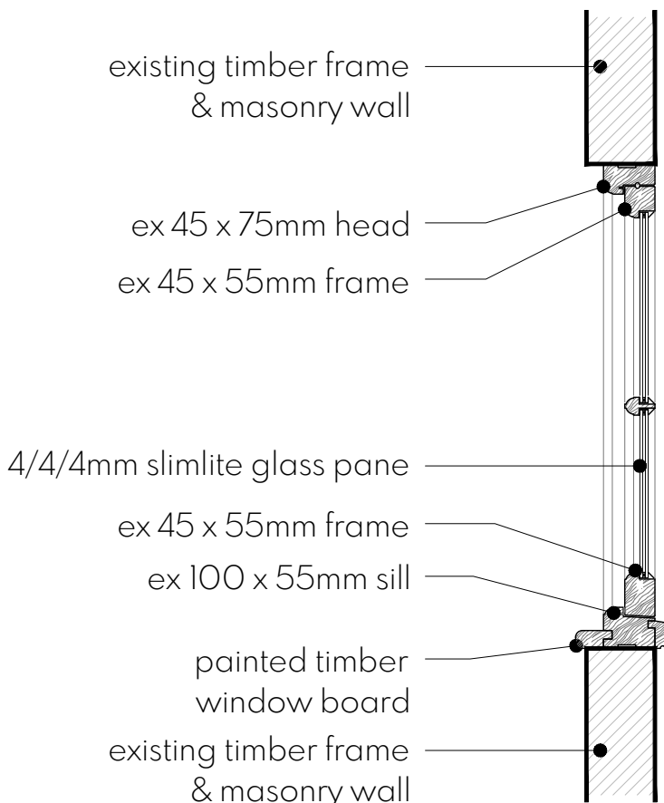
VERTICAL SECTION 1:10
