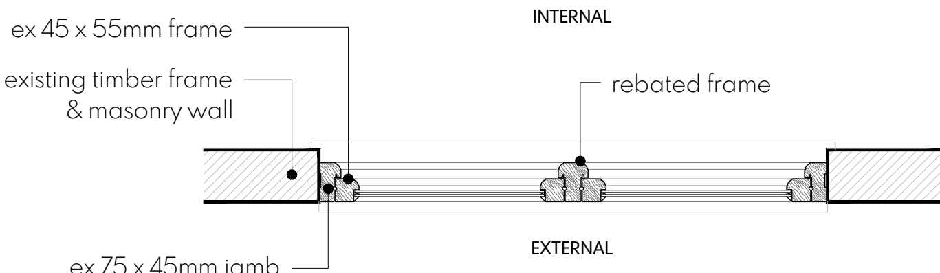
HORIZONTAL SECTION 1:10
