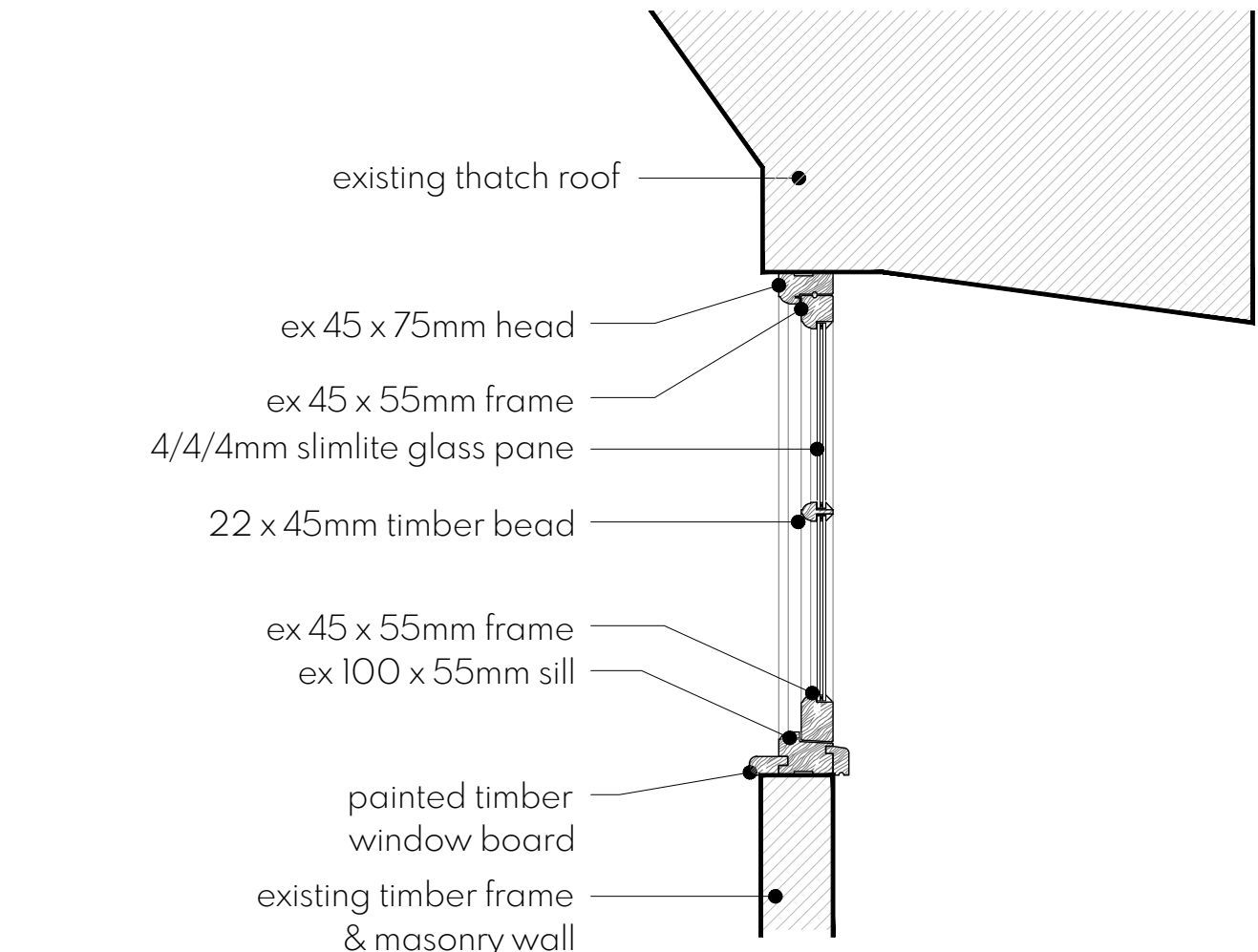
VERTICAL SECTION 1:10
