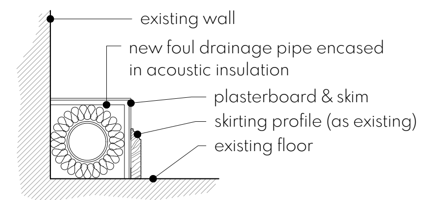
VERTICAL SECTION foul drainage pipe (100mm ø) 1:10
