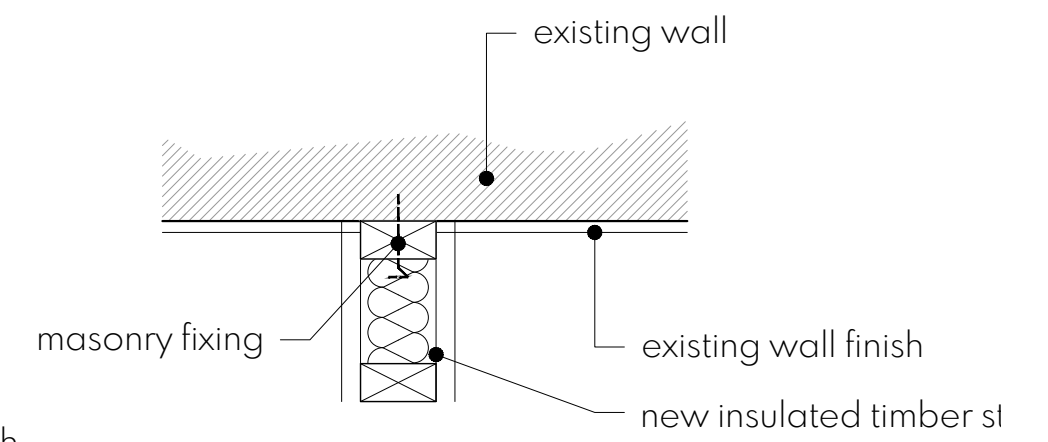
HORIZONTAL SECTION new studwork/masonry wall junction 1:10
