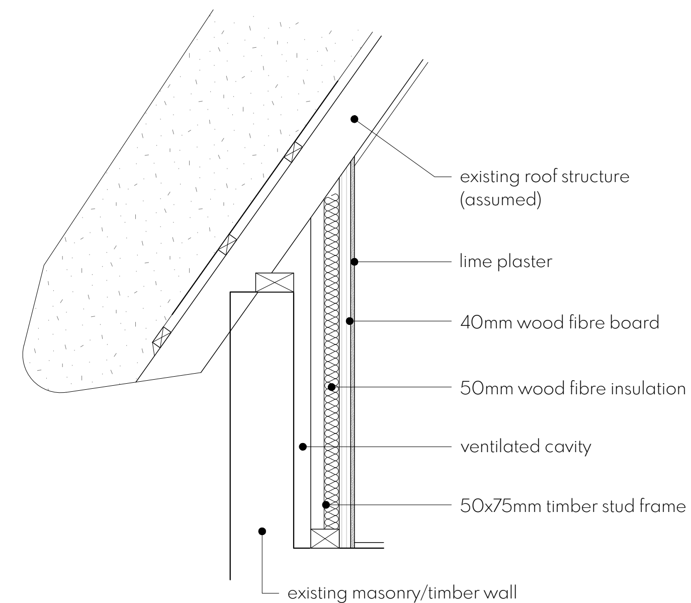
ENSUITE - INTERNAL INSULATION VERTICAL SECTION 1:10
