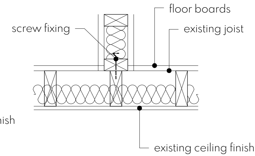
VERTICAL SECTION new studwork timber floor junction 1:10
