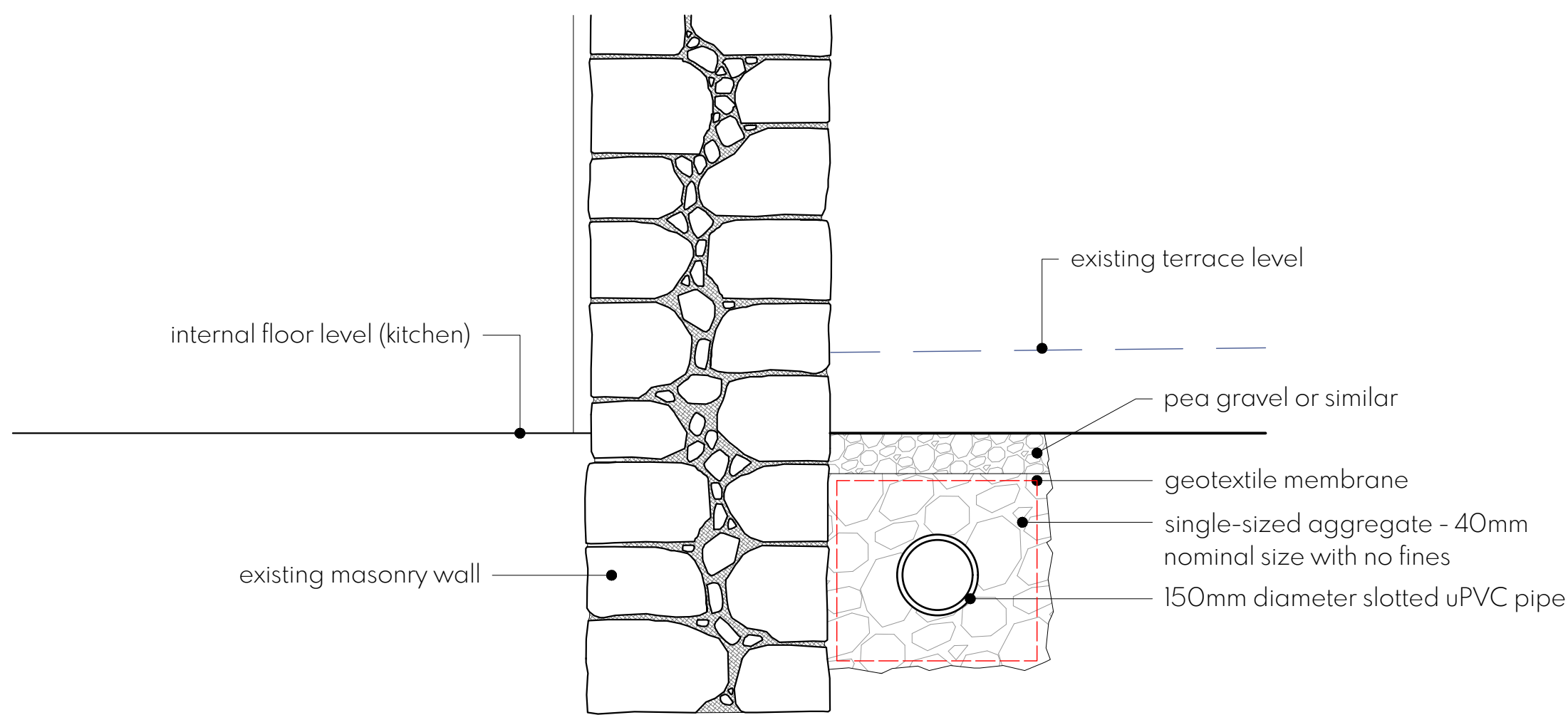
FRENCH DRAIN SECTION 1:10
