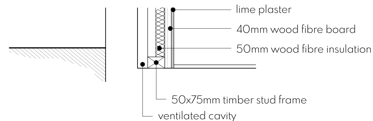
UTILITY - INTERNAL INSULATION VERTICAL SECTION 1:10
