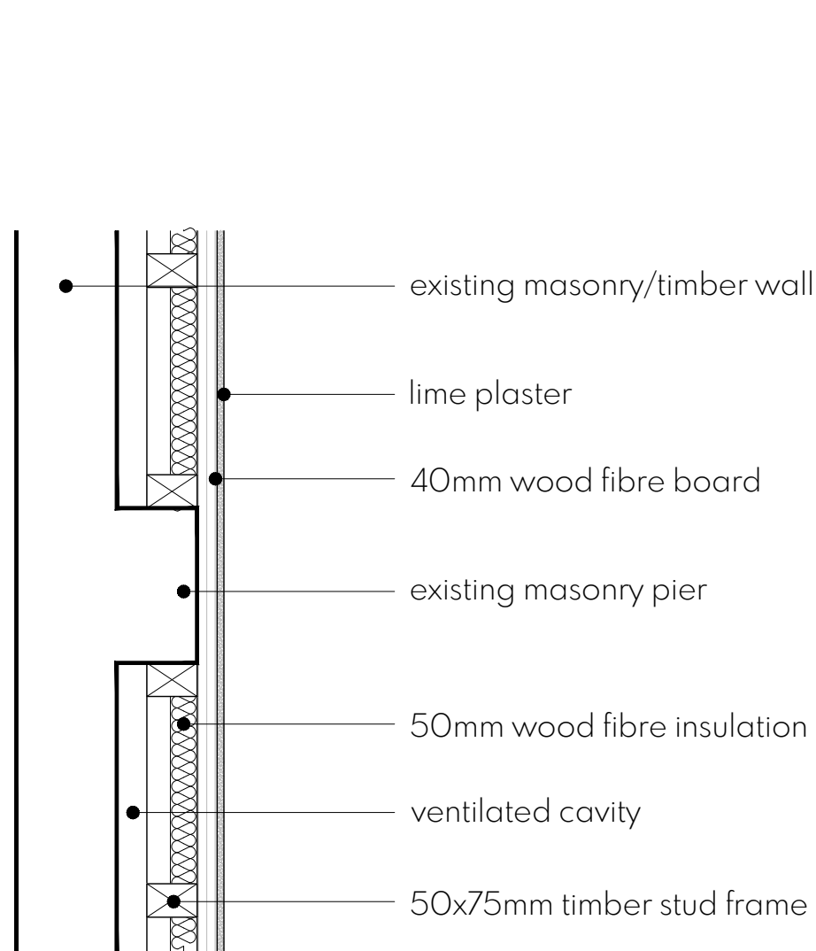
UTILITY - INTERNAL INSULATION HORIZONTAL SECTION 1:10
