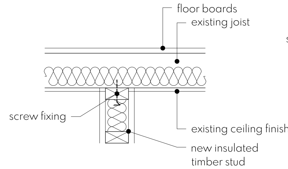
VERTICAL SECTION new studwork ceiling junction 1:10
