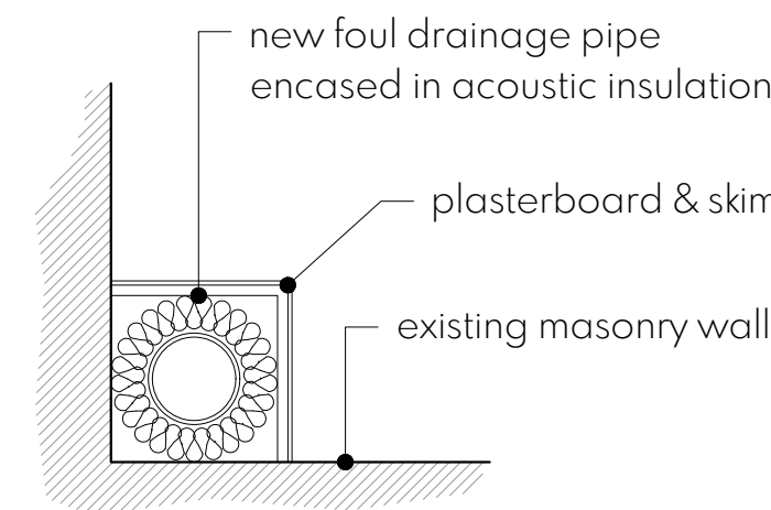
HORIZONTAL SECTION foul drainage pipe (100mm ø) 1:10
