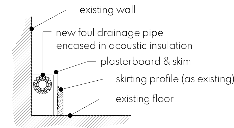
VERTICAL SECTION skirting boxing (40mm ø) 1:10
