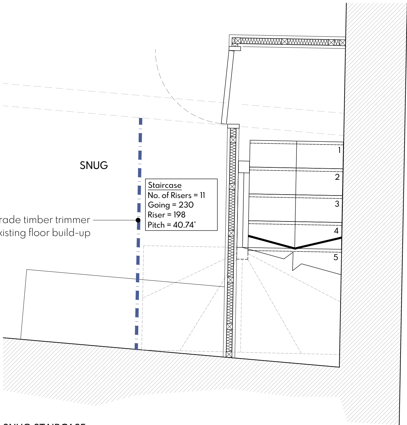
SNUG STAIRCASE Ground Floor Plan 1:20
