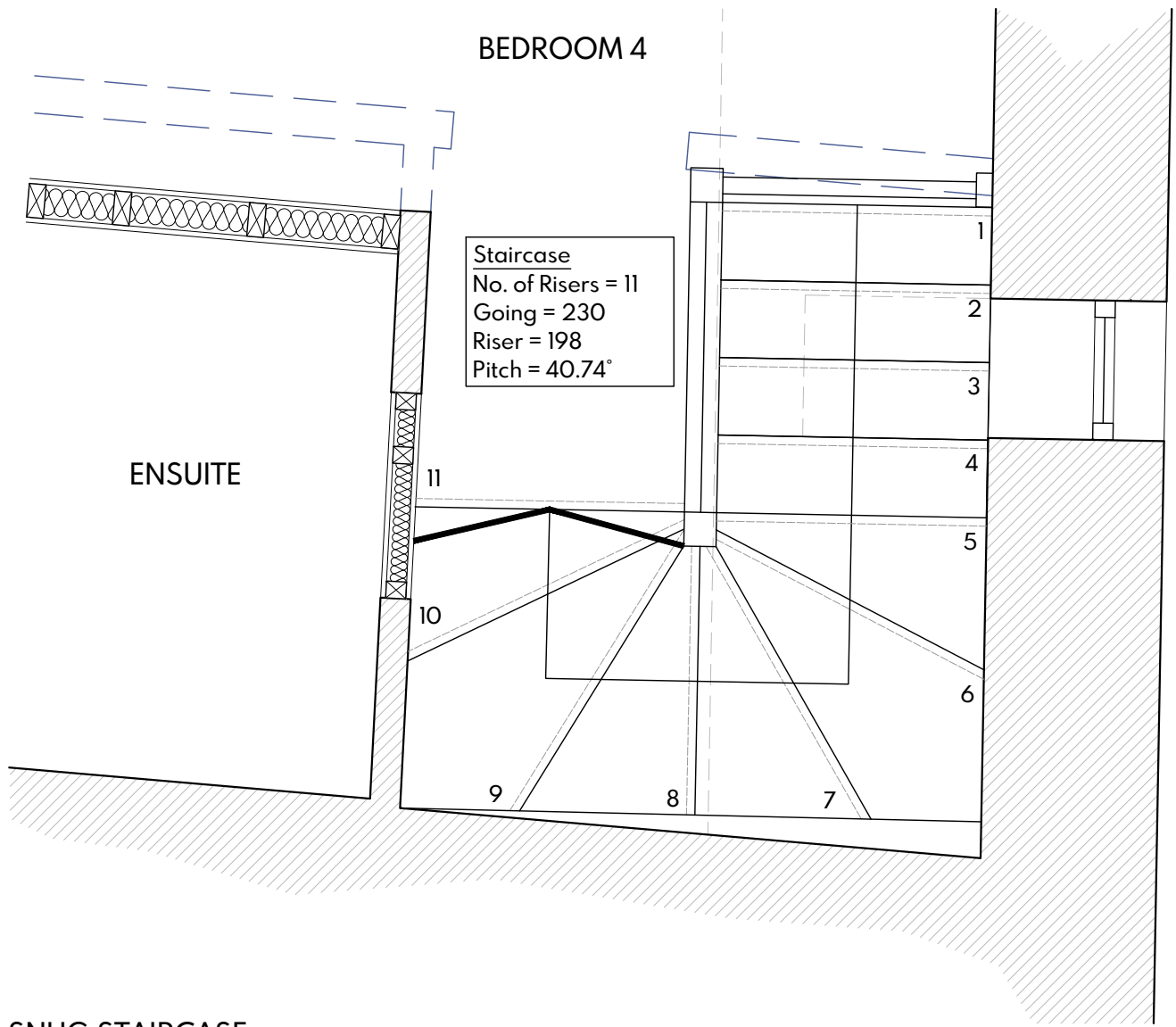
SNUG STAIRCASE First Floor Plan 1:20
