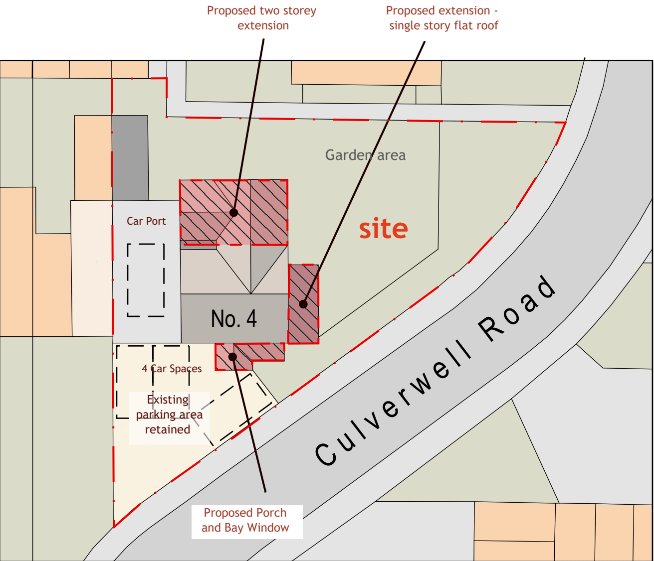
Proposed Layout
