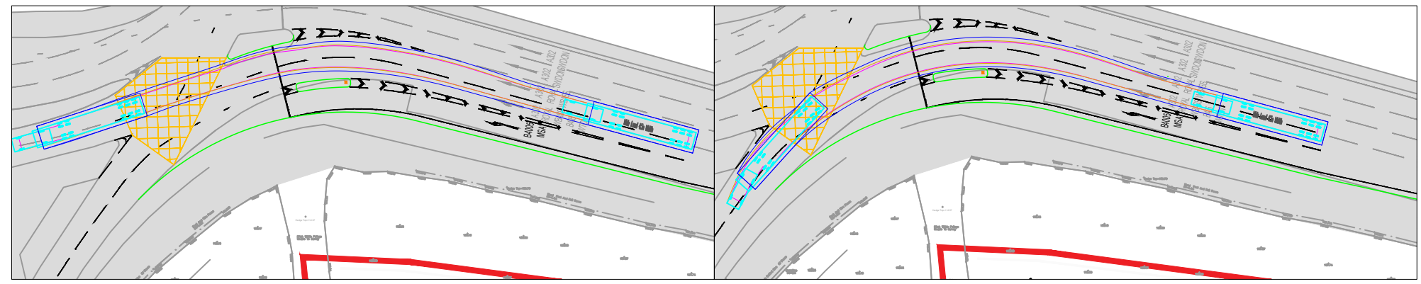
SWEPT PATH ANALYSIS: ABNORMAL LOAD VEHICLE (4.5M WIDTH)
