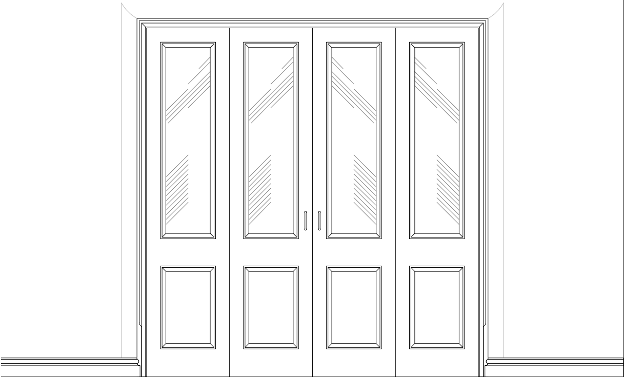
DG 01 Proposed bi-fold door Dining room elevation
