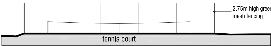
cross section
