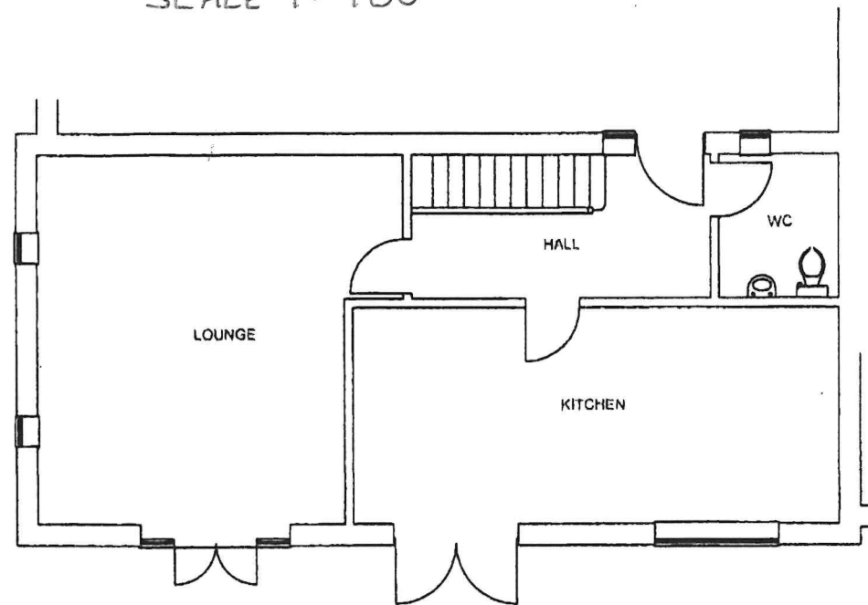
EXISTING FLOOR PLAN SCALE 1-100
