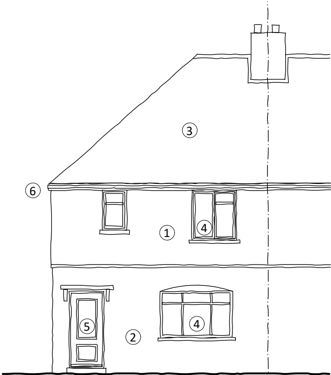
1:100 Existing North Elevation
